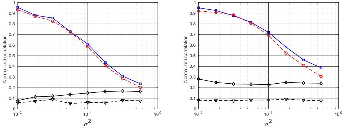
Fig. 1: Evolution of the (averaged) normalized correlation as a function of the variance \sigma^2 for K = 2 (left) and K = 5 (right), Comparison of the performance of conventionnal (delay-and-sum) beamforming (triangle mark), “prSAMP” (diamond mark), “paVBEM” (circle mark) and “paSAMP” (square mark). Experiments show that “paSAMP” provides better results and successfully integrates the phase noisy observation model.
