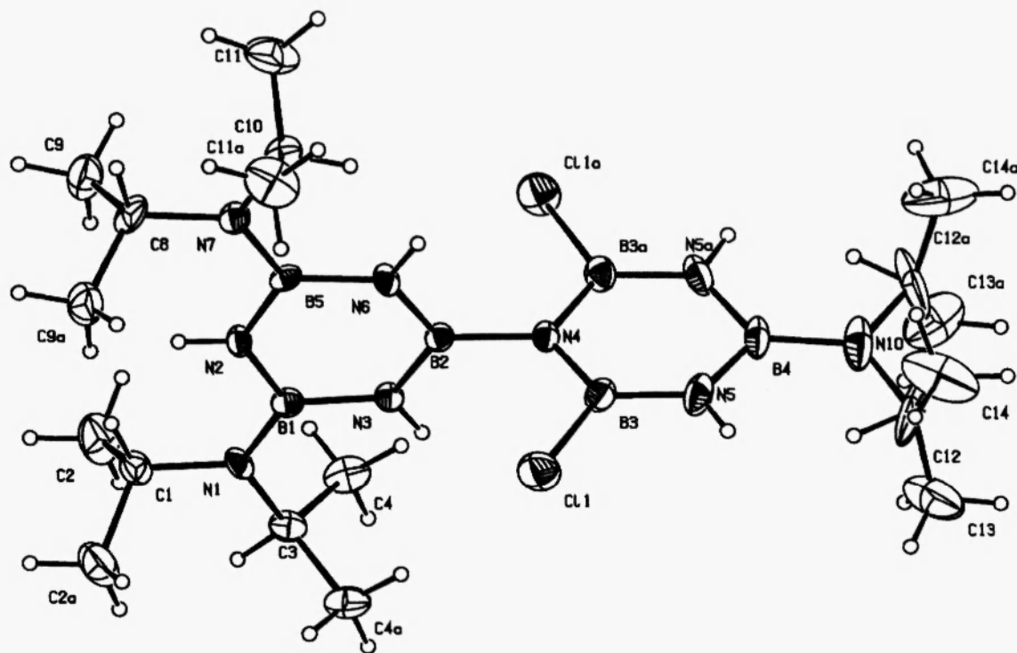
Figure 1. Molecular structure of the diborazine 1,2'-[(2,6-Cl 2 -4-(Pr i 2 N)B 3 N 3 H 3 )(4',6'-(Pr i 2 N) 2 B 3 N 3 H 3 )] 1 in the structure of the title compound. Selected bond distances (Å) and angles (°) for 1 : B-Cl 1.782(6), N(4)-B(2) 1.501(8), N(3)-B(2) 1.42(1), N(3)-B(1) 1.45(1), N(2)-B(1) 1.44(1), N(2)-B(5) 1.46(1), N(5)-B(3) 1.388(7), N(5)-B(4) 1.450(6), N(4)-B(3) 1.429(6), N(10)-B(4) 1.42(1), N(1)-B(1) 1.42(1), N(1)-C(1) 1.459(9), N(1)-C(3) 1.49(1), N(7)-B(5) 1.427(9), N(7)-C(8) 1.46(1), N(7)-C(10) 1.46(1), N(10)-C(12) 1.471(3), B(2)-N(3)-B(1) 123.4(6), B(5)-N(6)-B(2) 123.9(4), B(3)-N(4)-B(2) 122.6(3), B(3a)-N(4)-B(3) 114.7(5), N(3)-B(2)-N(4) 120.0(6), N(6)-B(2)-N(4) 121.4(6), B(3)-N(5)-B(4) 125.0(4), B(1)-N(2)-B(5) 125.0(5), N(1)-B(1)-N(2) 123.4(7), N(2)-B(1)-N(3) 114.2(6), N(2)-B(5)-N(7) 122.6(7), N(1)-B(1)-N(3) 122.3(7), N(3)-B(2)-N(6) 118.6(5), N(6)-B(5)-N(7) 122.5(6), N(2)-B(5)-N(6) 114.9(5), N(10)-B(4)-N(5) 124.7(3), N(4)-B(3)-N(5) 122.1(4), N(5)-B(4)-N(5a) 110.7(6).
