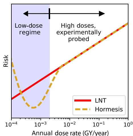
FIGURE 1 The Linear-No Threshold model, which describes the risk of cellular damage as linear with increasing dose is experimentally well validated for high doses, but is an extrapolation in the low-dose regime where biological responses are more difficult to probe. Alternative models, such as radiation hormesis, propose the hypothesis that small radiation doses are stimulatory and often beneficial, reducing the level of risk that would otherwise be present at zero dose
