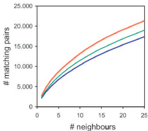
Figure 2. Number of predicted matching pairs for a given number of closest neighbors: old Phydbac (blue), new Phydbac2 (green), new Phydbac2 + chromosomal proximity (red).
