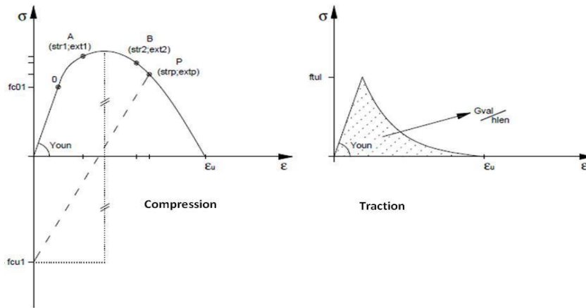
Figure 2-3 : DAMAGE_TC model in traction and compression
