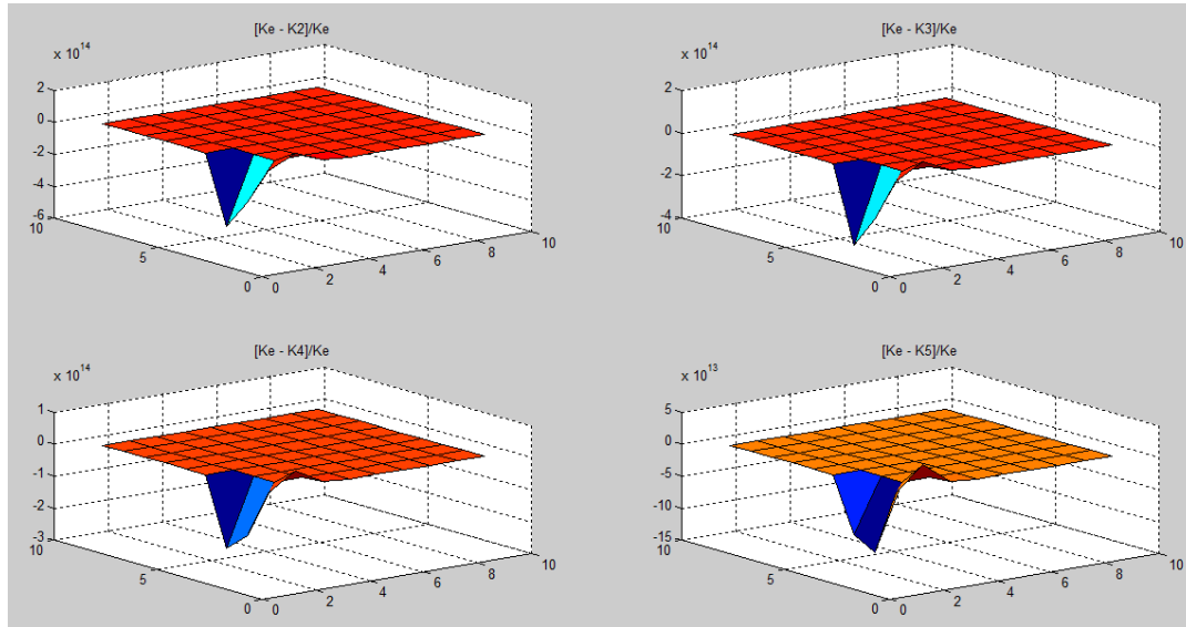
Figure 2-10 : Evolution of stiffness matrix degradations of the proposed macro-element
