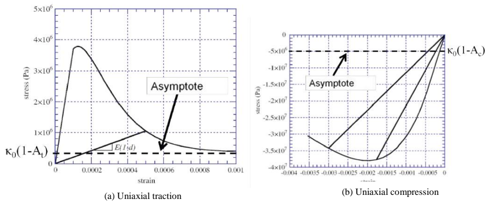
Figure 2-2 : Response of MAZARS model behavior under cyclic loading (Figure 2-3).
