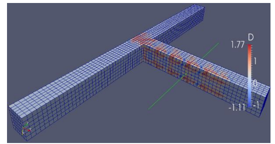
(b) DAMAG_TC (in traction)
