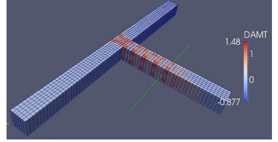
(b) DAMAG_TC (in traction)
