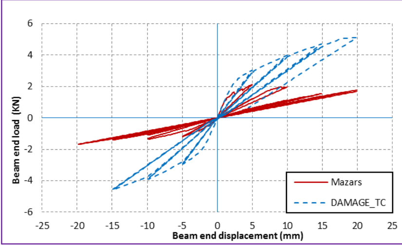
Figure 2-7 : Hysteretic behavior (cyclic loading)
