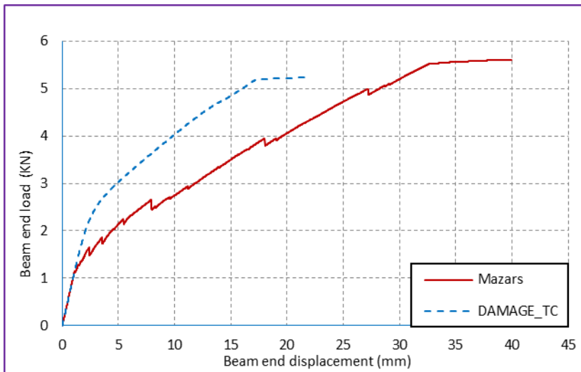
Figure 2-5 : Global response (monotonic loading)
