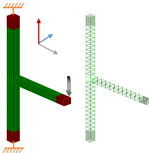
Figure 2-4: Modeling of exterior BC joint
