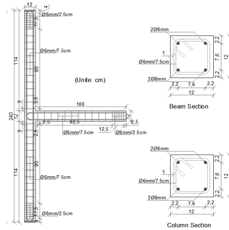
Figure 3-1: Reinforcement details of the
