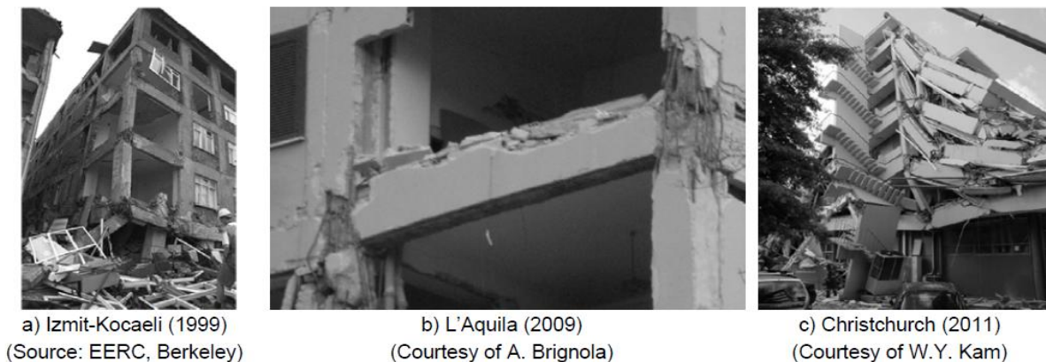
Figure 1-1: Joint failures in RC buildings during past earthquakes
