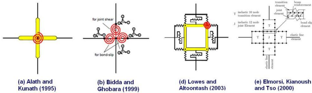
Figure 2-1: Macro-element models
