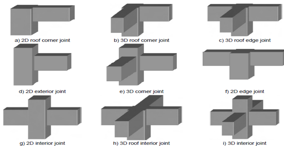
Figure 1-2: Classification of typical beam-column joints
