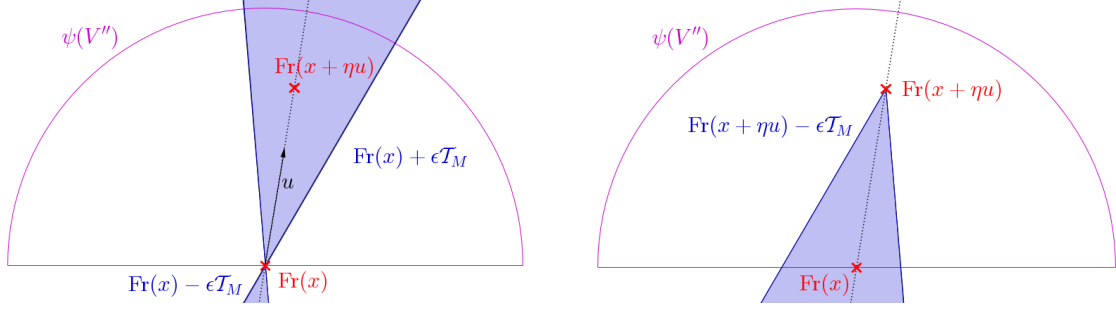
Figure 4.1: Proof of Lemma 4.18 when \dim H = 2 (the illustration is made in M )
