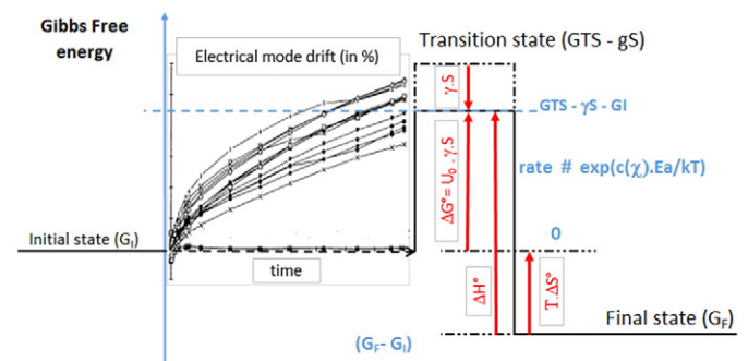
Fig. 4. Generalized BAZ model (Eq. (11)).
