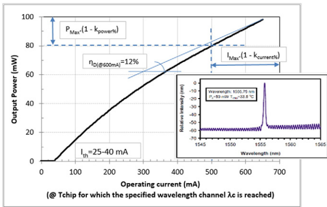
Fig. 2. Typical performance characteristics (P-I curve) of a 1550 nm DFB laser module from Manufacturer M.
