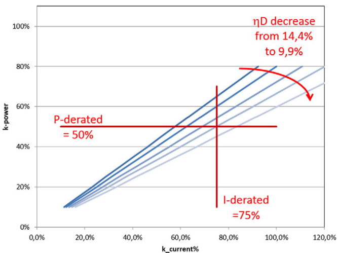
Fig. 3. Maximum rating limits and derating conditions (normalized w.r.t. maximum rating limits) required for high reliability application (effect of lot distribution due to lot Quantum Efficiency and threshold current dispersion).
