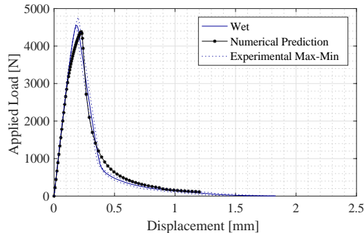
Figure 6. Calibration of model parameters
