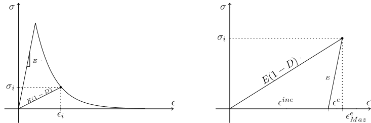
Figure 1. Uniaxial tension test with Mazars model
