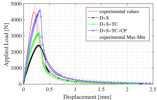
Figure 7. Prediction of the behaviour after drying
