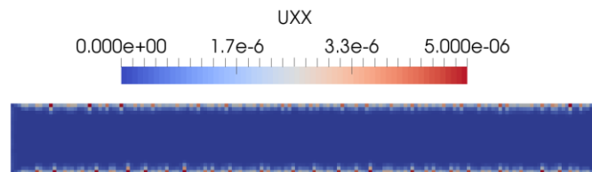
Figure 8. Crack map due to drying shrinkage [m]
