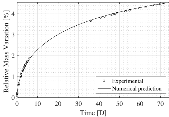
Figure 2. Evolution of Relative Mass Variation
