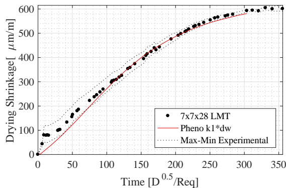
Figure 4. Evolution drying shrinkage
