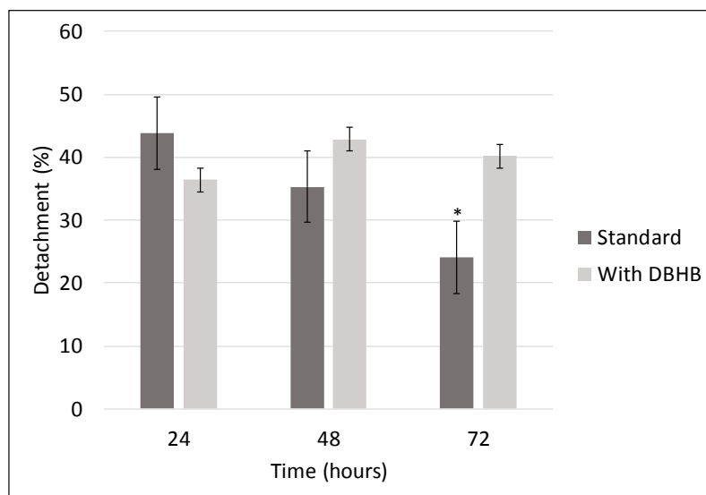
Figure 5. Impact of DBHB (16 \mu\text{M} ) on detachment of C. closterium after 24, 48 and 72 adhesion. Data represent the mean \pm standard deviation of replicates; * statistically significant difference at the 95% confidence level between standard (without DBHB) and treated samples.
