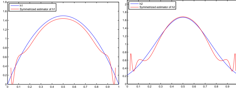
Figure 8: Reconstructions of h_1 (left) and h_2 (right) after symmetrization.
