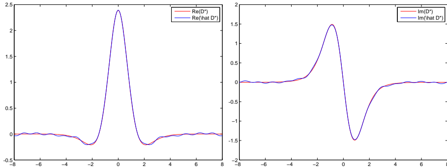
Figure 5: For the Beta(2, 2) density, the real part (left) and the imaginary part (right) of \widehat{\mathcal{D}}^* (blue line) compared with those of \mathcal{D}^* (red line).
