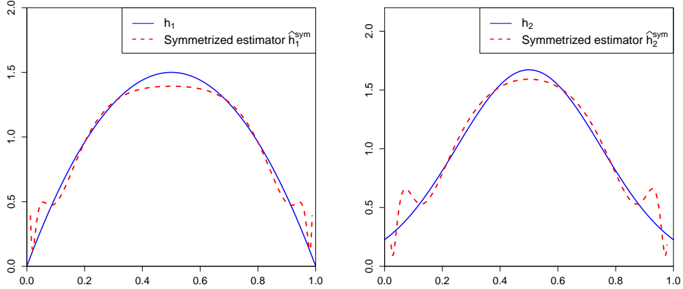
Figure 8: Reconstructions of h_1 (left) and h_2 (right) after symmetrization.
