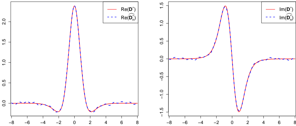
Figure 5: For the Beta(2, 2) density, the real part (left) and the imaginary part (right) of \widehat{\mathfrak{D}}_n^* (blue line) compared with those of \mathfrak{D}^* (red line).
