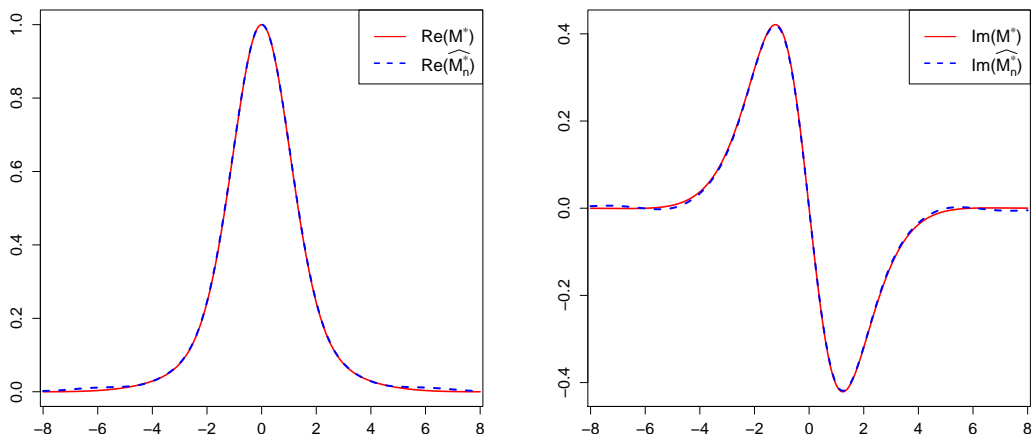
Figure 3: For the Beta(2,2) density, the real part (left) and the imaginary part (right) of \widehat{M}_n^* (blue line) compared with those of M^* (red line).
