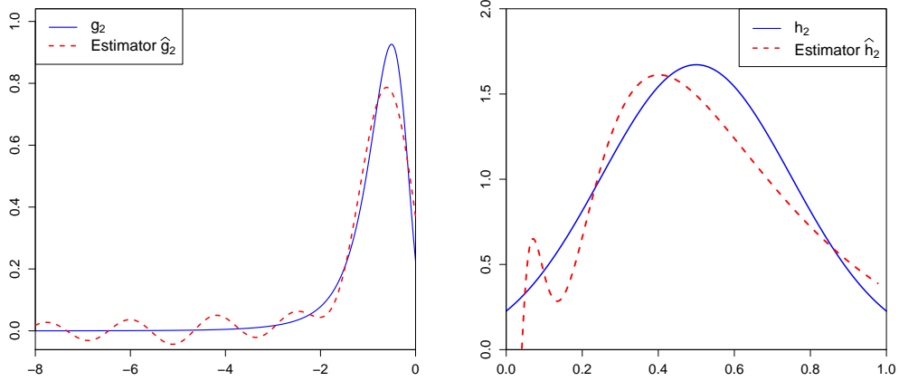
Figure 7: Estimation of g_2(x) = e^x h_2(e^x) (left) and h_2 (right).
