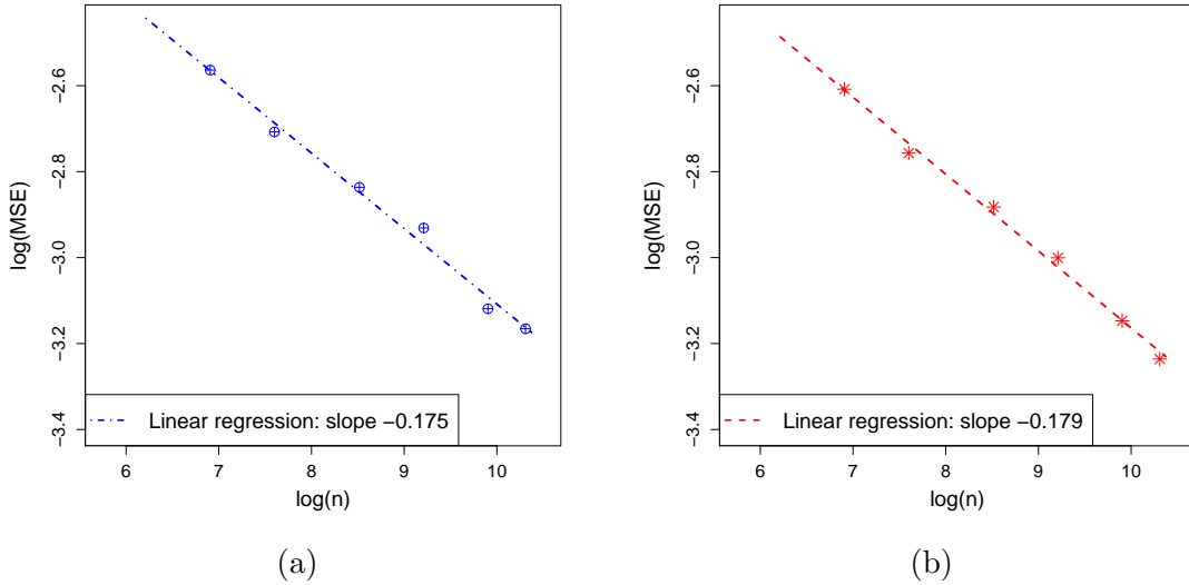
Figure 11: The regression lines for log-mean square error for the reconstruction of g_1 (left, Eq: y = -1.351 - 0.175x ) and the reconstruction of g_2 (right, Eq: y = -1.375 - 0.179x ) versus \log(n) , with the sample size n varying from 1,000 to 30,000.
