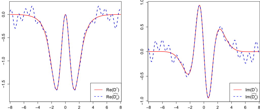
Figure 4: For the Beta(2, 2) density, the real part (left) and the imaginary part (right) of \widehat{D}_n^* (blue line) compared with those of D^* (red line).
