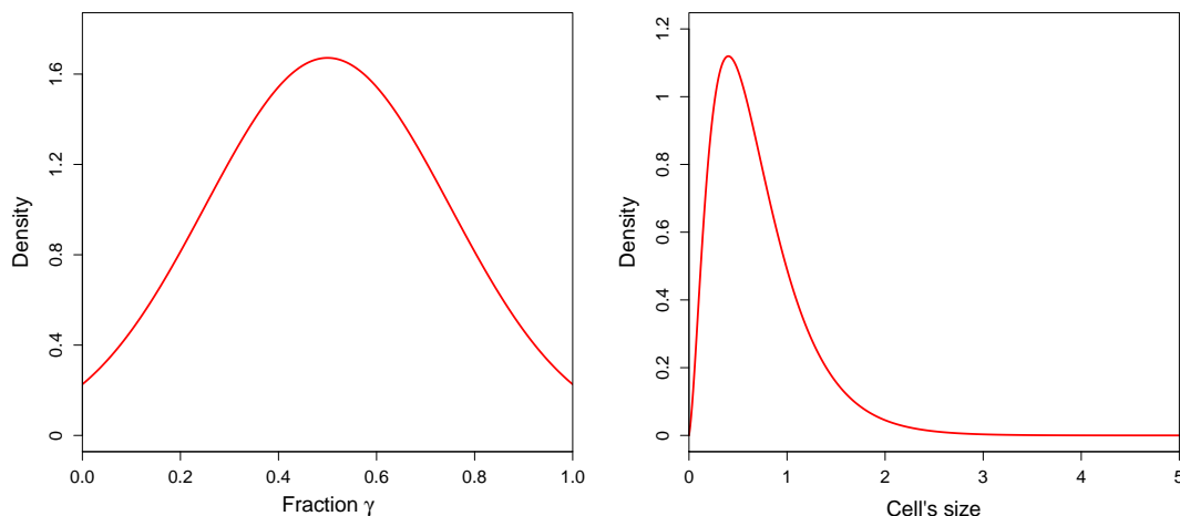
Figure 2: The truncated normal density h_2 (left) and its corresponding stationary density N_2 (right).
