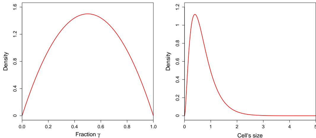
Figure 1: The Beta(2, 2) density h_1 (left) and its corresponding stationary density N_1 (right).
