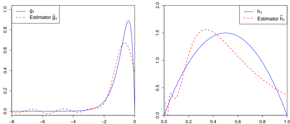
Figure 6: Estimation of g_1(x) = e^x h_1(e^x) (left) and h_1 (right).
