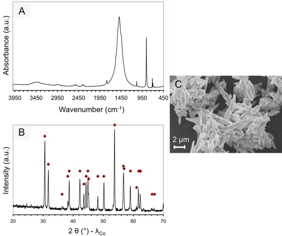
Fig. 1. Characteristics of aragonite crystals after crystal growth experiment at constant solution supersaturation and in absence of orthophosphate ions: FTIR spectrum (a), powder X-ray diffractogram (b, rhomboid symbols show the aragonite seeds diffraction peaks assigned in comparison with the JCPDS n° 411475 reference data) and SEM micrograph (c).
