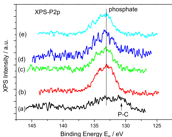
Fig. 7. XPS spectra of aragonite crystals equilibrated with orthophosphate solutions. (a) blank (b) 1.3 \mu\text{mol m}^{-2} (c) 6.6 \mu\text{mol m}^{-2} (d) 13.6 \mu\text{mol m}^{-2} (e) 21.6 \mu\text{mol m}^{-2} .
