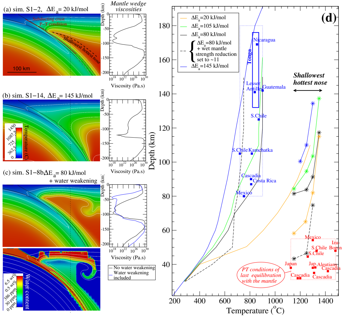
Figure 13: (a-c) Subduction thermal structures at steady-state as a function of \Delta E_a . One white isotherm every 200 ^{\circ} C. The black outline delimits the subducting crust. Thermal states modelled with \Delta E_a = 80 kJ/mol and \Delta E_a = 105 kJ/mol are displayed in Fig. 3a and 4c. Right panels display viscosity profiles along the dotted line depicted in left panels. (d) P-T conditions modelled along the subducting crust surface (solid lines) compared to slab surface temperature estimated by geothermometry (Plank et al., 2009; Cooper et al., 2012; Watt et al., 2013) and sub-arc slab surface depth from Syracuse and Abers (2006) (blue solid squares, blue-dotted box). Lines with stars depict the hottest geotherm modelled in the mantle wedge, compared with conditions of last equilibration with the mantle of near-primary arc magmas (Tatsumi, 1981; Tatsumi et al., 1983; Bartels et al., 1991; Draper and Johnston, 1992; Falloon and Danyushevsky, 2000; Elkins Tanton et al., 2001; Grove et al., 2003; Hesse and Grove, 2003; Watt et al., 2013, red solid squares, red-dotted box).
