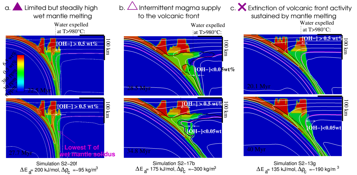
Figure 10: Prediction of water amounts (labelled [OH - ]) available in the mantle wedge to sustain mantle melting, for a 20 Myr old downgoing plate. Purple symbols in headings refer to Fig. 9a. (a) Water absorbed in the mantle wedge at temperature exceeding the minimum wet solidus temperature ( 980^\circ\text{C} , pink isotherm) in amounts always > 0.5\text{wt}\% sufficient to allow continuous melting. (b) Water absorbed at T > 980^\circ\text{C} in amounts strongly varying through time, temporarily very low and yielding discontinuous magmatism in the mantle wedge. (c) Progressive decrease through time of the water amount absorbed at T > 980^\circ\text{C} , predicting mantle melting to vanish off.
