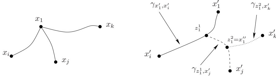
Figure 3: One maps \text{c\ddot{o}r}e(G) to \text{c\ddot{o}r}e(G') by first mapping the neighborhood of each vertex of \text{c\ddot{o}r}e(G) to a subset of G' . Here x''_1 is a vertex of \ker(G') .
