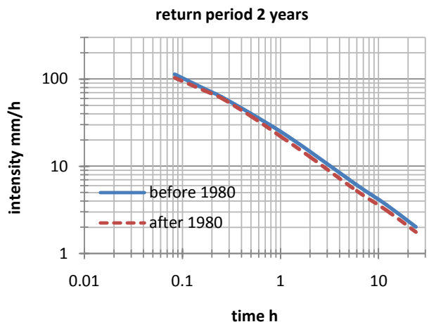
Figure 3. IDF curves before and after 1980. T = 2 years.
