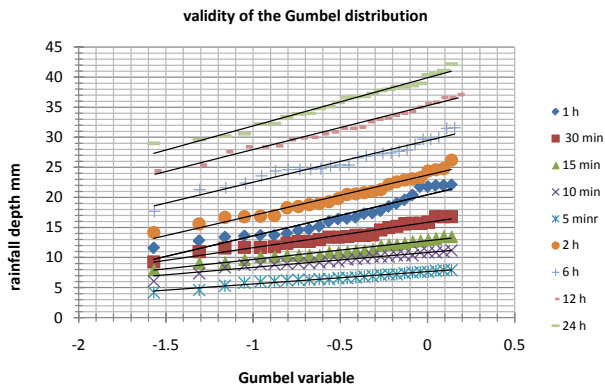
Figure 2. Validity of the Gumbel distribution.
