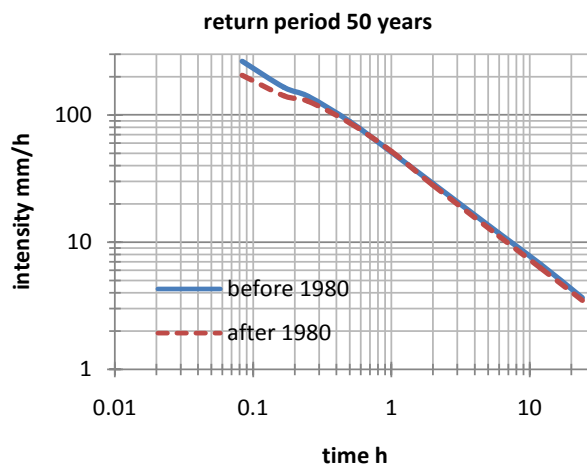
Figure 7. IDF curves before and after 1980. T = 50 years.
