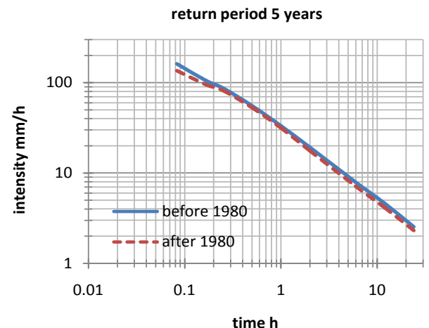
Figure 4. IDF curves before and after 1980. T = 5 years.
