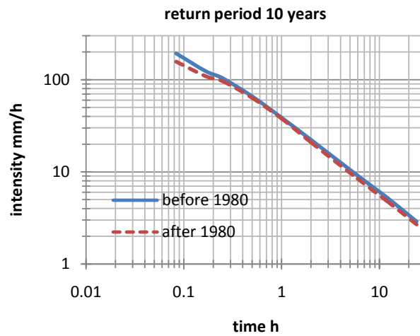
Figure 5. IDF curves before and after 1980. T = 10 years.
