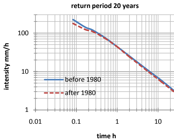
Figure 6. IDF curves before and after 1980. T = 20 years.
