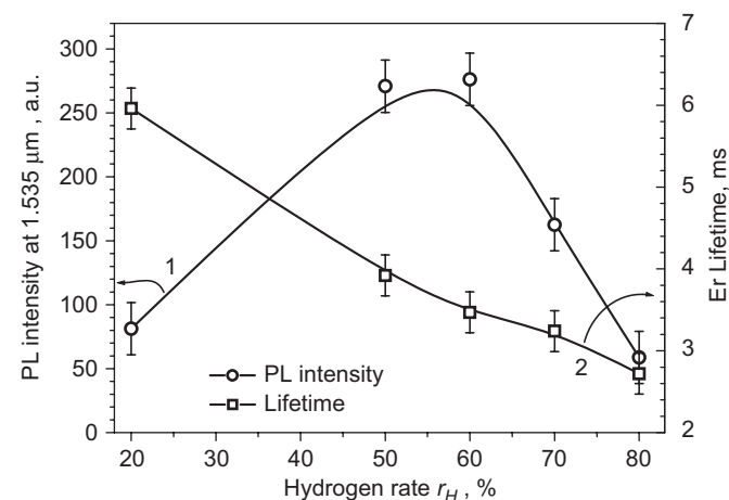
Fig. 1. Dependence of Er 3+ PL intensity (curve 1) and lifetime (curve 2) of SRSO-Er layers deposited at T_s = 100 °C on the hydrogen rate r_H . The measurements were made by using the non-resonant excitation line (476 nm).
