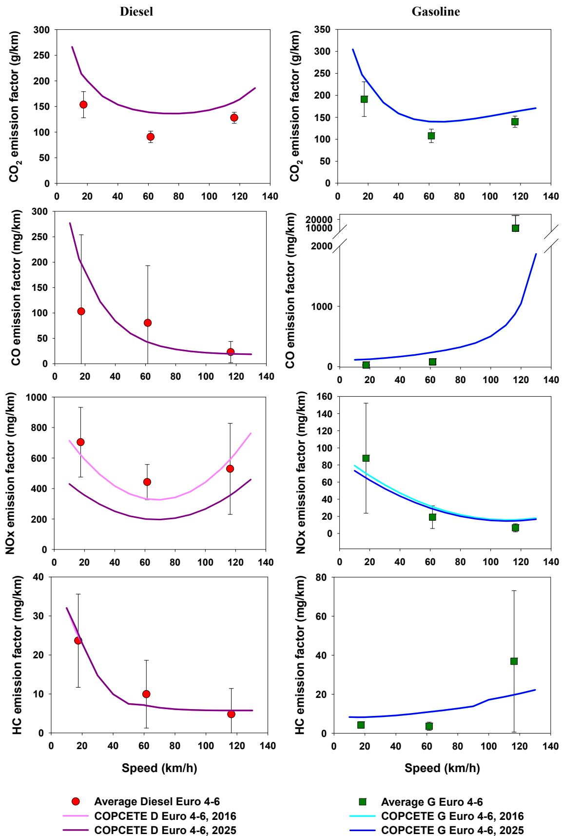
Fig. 3. Comparison between average emission factors for Euro 4–6 diesel (left) and gasoline (right) vehicles measured using Artemis urban, road and motorway hot start driving cycles and the COPCETE model prediction for the 2016 (pink and light blue) and 2025 fleets (purple and dark blue).
