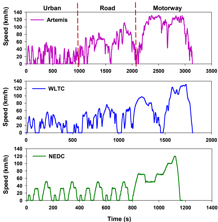
Fig. 1. Artemis Urban, Road and Motorway, WLTC and NEDC driving cycles.
