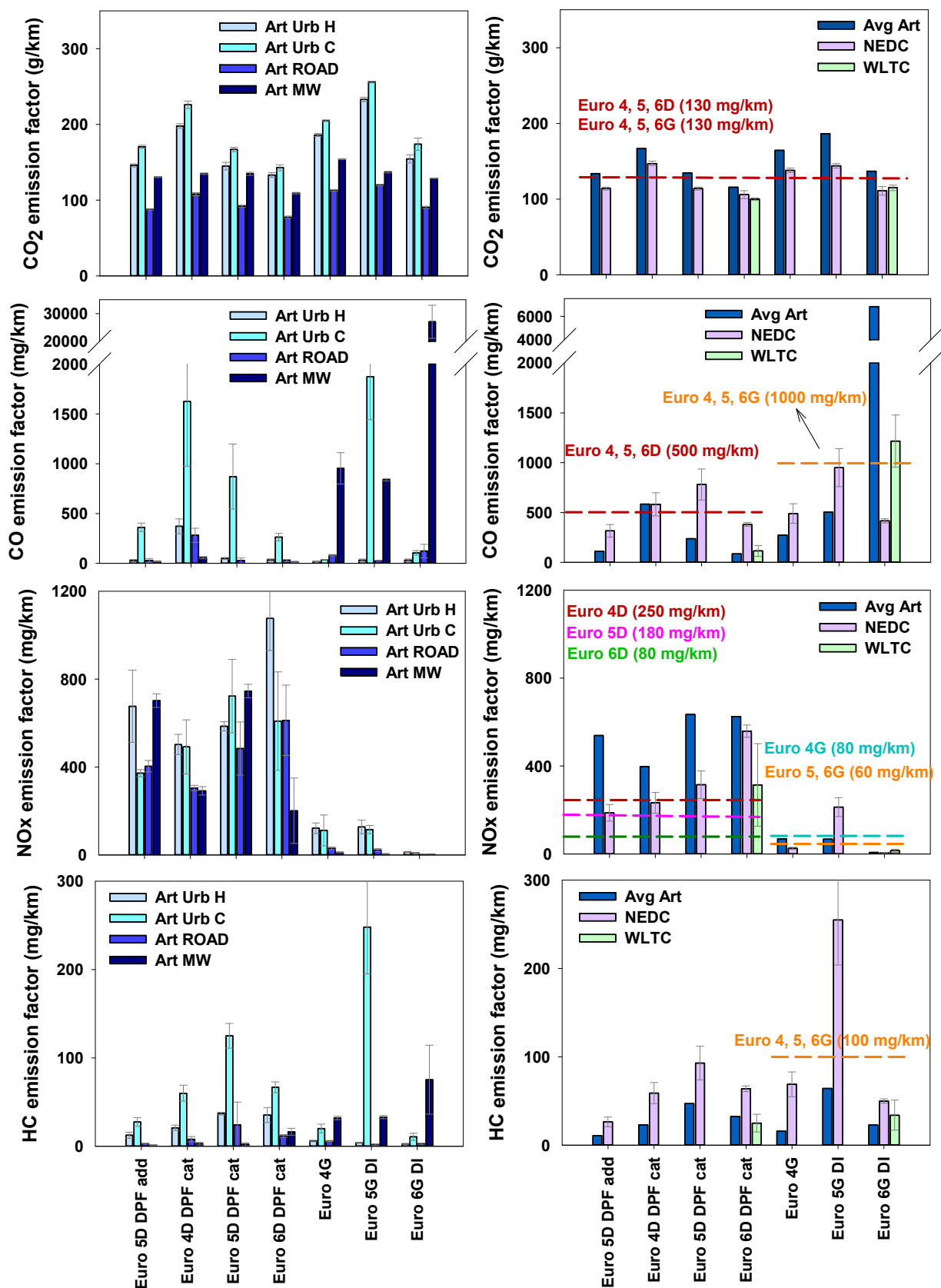
Fig. 2. CO 2 , CO, NO x and HC emission factors obtained under Artemis Urban with hot (Art Urb H) and cold start (Art Urb C), Road (Art ROAD) and Motorway (Art MW) driving cycles (left) and comparison of Artemis average emissions (Avg Art) with NEDC and WLTC emissions (right) for all the tested vehicles. The dotted lines denote Euro 4, 5 and 6 emission standards for diesel and gasoline vehicles.
