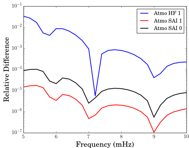
Fig. 6: Relative difference between the reflection coefficients as a function of frequency. The different boundary conditions are compared relatively to the (Reference) BC. A phase speed filter centered at 250.4 km/s is used in all cases.
