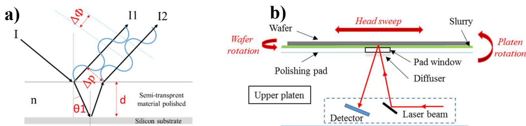
Fig. 2: a) depicts the interferometry principle for the simple case of two reflected beams on a SiO 2 layer above a silicon substrate. I is the incoming beam intensity from the laser source and it is both reflected on the semi-transparent material
