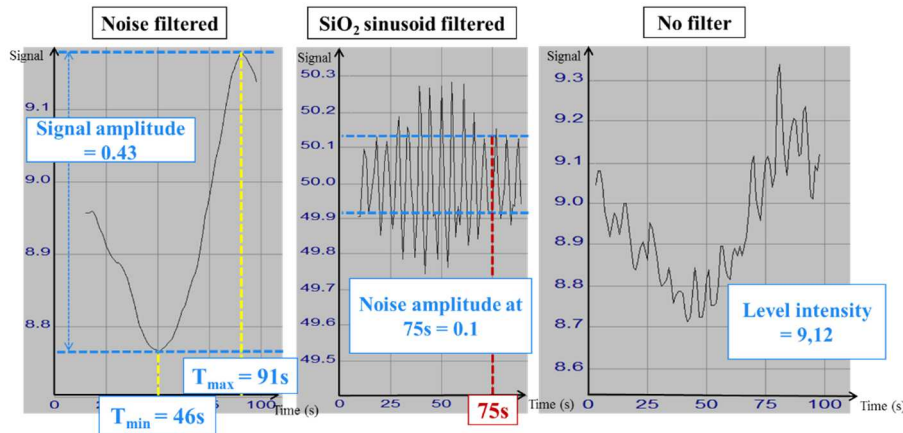
Fig 5: Responses associated with the D-Optimal plan. T min , T max and the signal amplitude are determined from the SiO 2 removal curve with noise filtering. On the contrary, the noise amplitude is given by filtering the SiO 2 removal curve. Finally, the intensity level is determined without any filter
