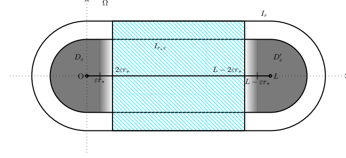
Figure 2: Illustration of the interval I and both its r and (r_*\varepsilon) -enlargement for r_* \geq 1 . In grayscale we plot the levels of the function \zeta_\varepsilon , whilst the striped region corresponds to the cylinder C_{r,\varepsilon} .
