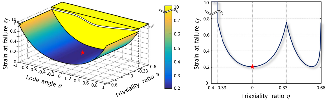
Fig. 6. (a) Shape of the identified fracture locus in the (\epsilon_f, \eta, \theta) space at T = 20^\circ\text{C} and a rate of 1\text{ mm s}^{-1} . (b) Restriction to the plane stress case. The calibration point is depicted as a red star ( \epsilon_f = 0.213 ). (For interpretation of the references to color in this figure legend, the reader is referred to the web version of this article.).
