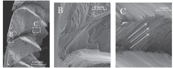
Fig. 17. SEM view of the chip ( V_c : 25 \text{ m min}^{-1} , rake angle 15^{\circ} ), B: detail view of crack, C: detail of crack orientation.
