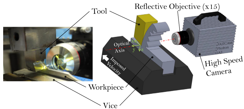
Fig. 10. Experimental setup.
