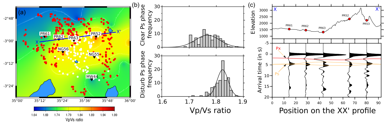
Figure 9. Insert a: seismic piercing points at Moho depth superimposed on the Vp/Vs map zoomed in the Crater Highlands area (Fig. 6). The red points are piercing points with a clear and regular Moho signature in the RFs, while white points are piercing points associated with disturbed Ps peak within the RFs. Insert b: distribution of Vp/Vs ratio according to the quality of the Ps peak (clear on top, disturbed at bottom). Insert c: stacked RFs for stations located on the Crater Highlands along the XX' profile (insert a).
