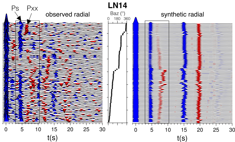
Figure 7. Left: observed radial RFs for LN14 organized by increasing backazimuth (Baz). Converted phases at the Moho (Ps, positive) and at the mantle discontinuity (Pxx, negative) are labelled. Right: corresponding synthetic radial RFs computed with Frederiksen & Bostock (2000) method. The model is composed of a 39 km thick crust ( V_p = 6.68 \text{ km s}^{-1} , V_p/V_s = 1.74 ), an upper mantle layer (30 km thick, V_p = 8.1 \text{ km s}^{-1} , V_p/V_s = 1.8 ), and an LVZ with V_p = 7.4 \text{ km s}^{-1} , V_p/V_s = 1.8 , a dip angle of 30^\circ and a strike of N40^\circ .
