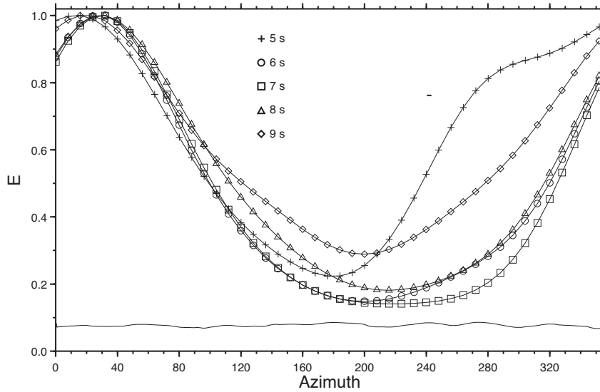
Figure 3. Normalized noise energy E as a function of propagation azimuth ( \theta ) for periods between 5 and 9 s. Maximum 2\sigma uncertainties are \sim\pm 9 per cent for the periods analysed and are shown as a function of azimuth by the solid line near the bottom of the figure. Note that the peak in this period range is at about 30^\circ , meaning that most of the noise recorded by the CRAFTI-CoLiBrEA network propagates along the rift valley from SSW to NNE.
