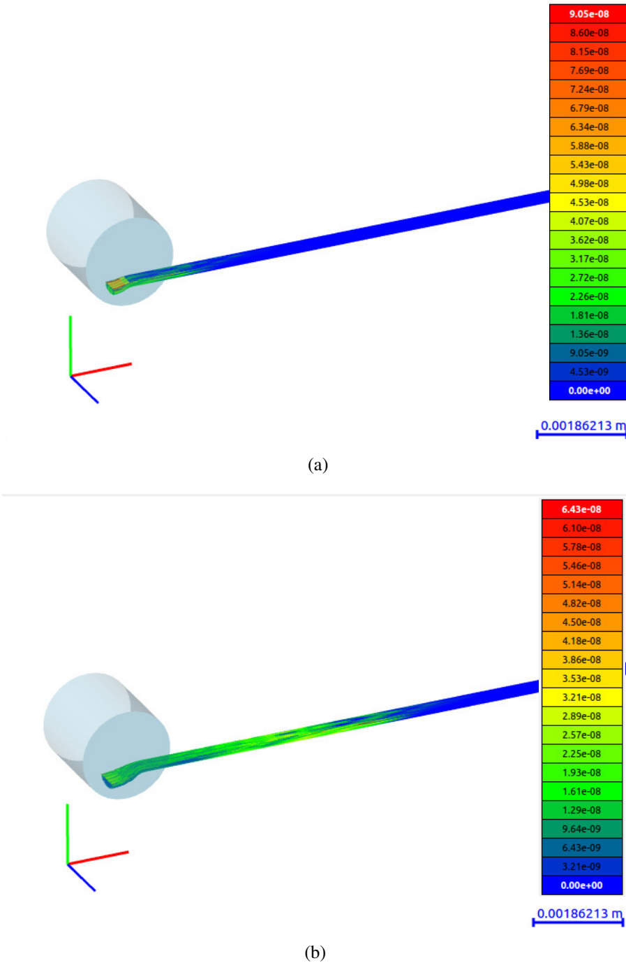
Fig. 10. Internal energy of the yarn [J] at 0.6 \mu\text{s} (a), 1.2 \mu\text{s} (b)
