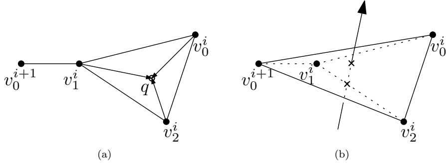
Figure 4: Illustration of lemma 2. In (a), the plane passing by \vec{v}_1^i, \vec{q}, \vec{v}_2^i separates \vec{v}_0^i from \vec{v}_0^{i+1} . In (b), a ray that goes inside the tetrahedron through edge [\vec{v}_1^i \vec{v}_2^i] must exit through a point of a facet that is not \mathbf{T}^{(i+1)} .
