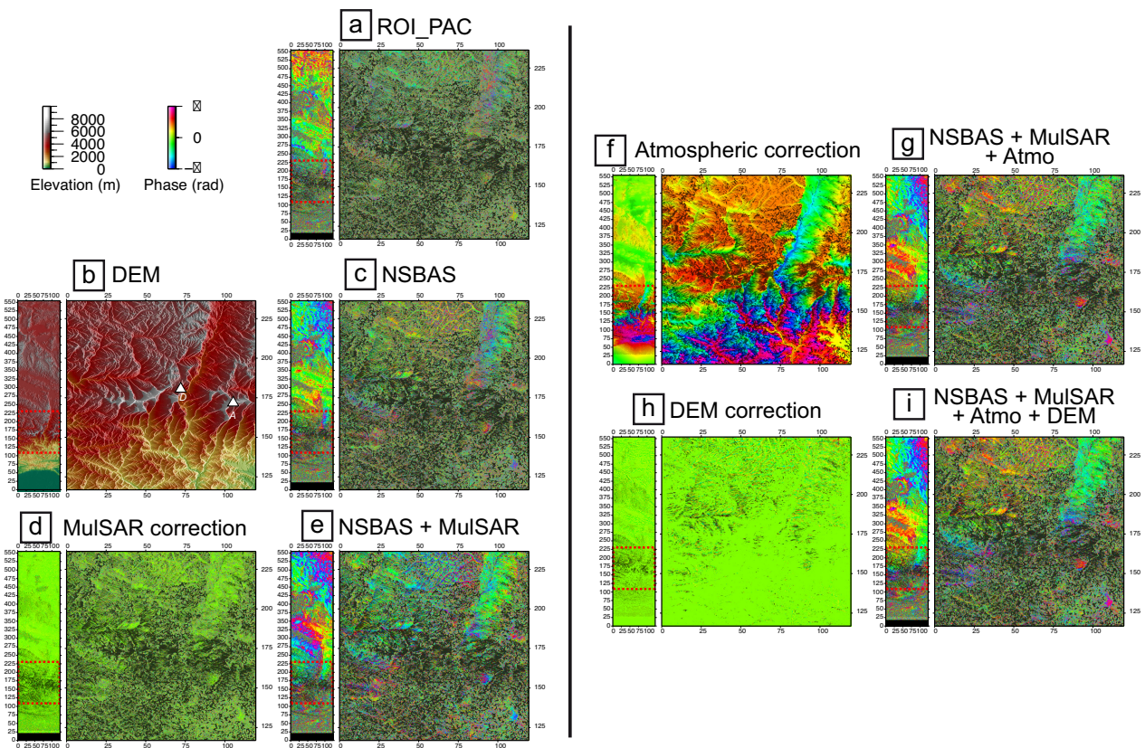
Figure S-3: Example of the effect of successive corrections applied prior to phase unwrapping. The example corresponds to an interferogram between 2006/12/27 and 2010/01/20 which was used in the stack. The temporal baseline of the interferogram is 3.06 years, and its perpendicular baseline is 236 m, which correspond to unfavourable conditions in terms of interferometric coherence. For each step, in order to highlight the impact of corrections on a broad scale and on a small scale, the interferogram spanning the whole swath (see Figure S-1 for location) is shown to the left of a blow up on the area with greatest topographic relief centered on the Himalaya (area surrounded by red dashed box). Areas in black in interferograms are incoherent regions where corrections are inefficient. (a) Interferogram processed with ROI_PAC. (b) SRTM-DEM in radar geometry. A: Annapurna. D: Dhaulagiri. (c) Interferogram processed with NSBAS [Doin et al., 2011]. (d) Correction for this interferogram determined after Multi-link InSAR time series (MulSAR) processing [Pinel-Puysségur et al., 2011]. (e) Interferogram after MulSAR correction. (f) Tropospheric delay correction computed from the ERA-Interim atmospheric model [Jolivet et al., 2011]. (g) Interferogram after atmospheric correction. (h) DEM correction calculated from combination of (wrapped) coherent interferograms with large perpendicular baselines and small temporal baselines [Ducret et al., 2011]. (i) Interferogram after DEM correction. Note the substantial improvement of the coherence between (a) and (i).
