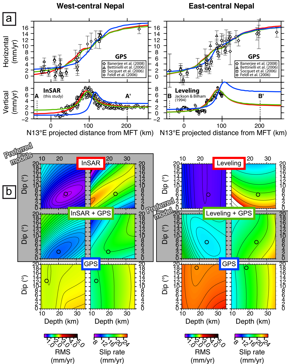
Figure S-11: (a) Horizontal (top) and vertical (bottom) components of interseismic velocity field across the Himalaya in West-Central Nepal (left) and East-Central Nepal (right). The location of profiles is indicated by the red and green boxes in Figure S-10. (b) Exploration of fault parameters using a dislocation model for the two sub-regions using different data sets as input for the inversions. For each given depth and dip of the dislocation, we invert for the optimal fault slip rate and fault location along the profile. Top panels show inversion results using vertical data only (InSAR or leveling), bottom panels show inversion results using horizontal data only (GPS), and middle panels are for joint inversion of horizontal and vertical data. In each panel, the left plot is the root-mean-square (RMS) of the residual, and the right plot is the slip rate determined for each inversion. Color dots indicate the minimum RMS location for the simultaneous inversion of the full set of parameters. Horizontal and vertical surface velocity fields predicted by each inverted fault model are shown in (a). Red: vertical only; blue: horizontal only; green: vertical and horizontal. The preferred models are highlighted by a grey box.
