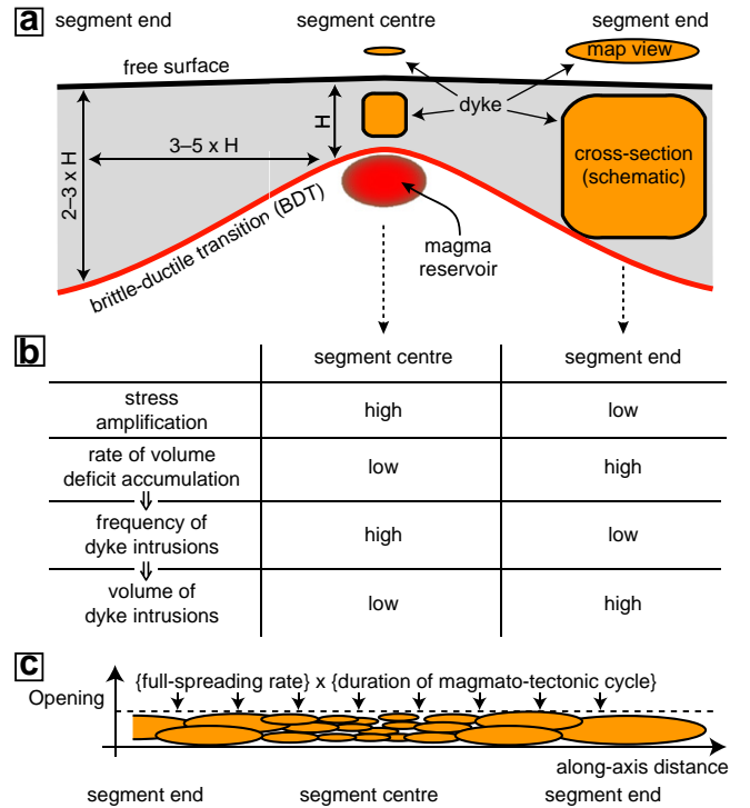
Fig. 7. (a) Dykes emplaced near segment centre are thinner, shorter and smaller than those intruded at segment ends because of scaling laws and the limit imposed by the local thickness of the elastic–brittle lithosphere. (b) For a constant spreading rate, stress builds up at a faster rate near segment centre because of stress amplification, but less magma volume is required to accommodate spreading on the long run. Hence, frequent, small volume dykes are required. Conversely, dyke intrusions are less frequent near segment ends, but their volume is significantly larger. (c) Frequent, thin dykes near segment centre, and infrequent, thick dykes near segment ends can maintain a constant rate of opening and a steady-state accretion.
