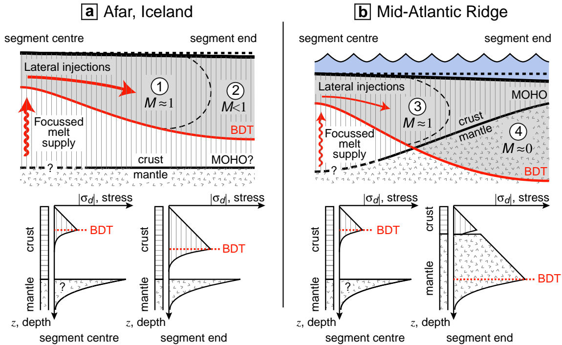
Fig. 6. Along-axis cross-sections showing two different configurations of the thermal and compositional structure of the lithosphere leading to along-rift deepening of the brittle ductile transition (only half of the segment length is shown here). M is defined as the fraction of the plate separation rate accommodated by magmatic dyke opening (e.g. Buck et al., 2005). Diagrams at the bottom indicate the inferred distribution of the absolute value of differential stress |\sigma_d| as a function of depth near segment centre and near segment ends. (a) In Afar and Iceland, the BDT is likely to be shallower than the crust–mantle boundary (MOHO), due to the anomalously thick Icelandic crust (e.g. Allen et al., 2002), and the transitional nature of the Afar crust (e.g. Makris, 1987; Sicilia et al., 2008; Tiberi et al., 2005), respectively. Deepening of the BDT within the crust, due to a colder geotherm away from the source reservoir, promotes lateral dyke injections, but other factors prevent lateral dyke migrations over large distances, such as pressure drop in the magma or stress shadows inherited from previous intrusions. M is therefore near to 1 at the segment centre (1), and decreases toward segment ends (2). (b) In a mid-ocean ridge segment, regular access of magma to proximal sectors of the magmatic segment also ensures a sustained magmatic accretion (3). However, the relatively less robust magma supply yields a low M in remote sectors of the segment, thus implying that faulting accommodates a greater fraction of plate extension (4), possibly explaining the more pronounced rift valley topography in comparison to sub-aerial rifts.
