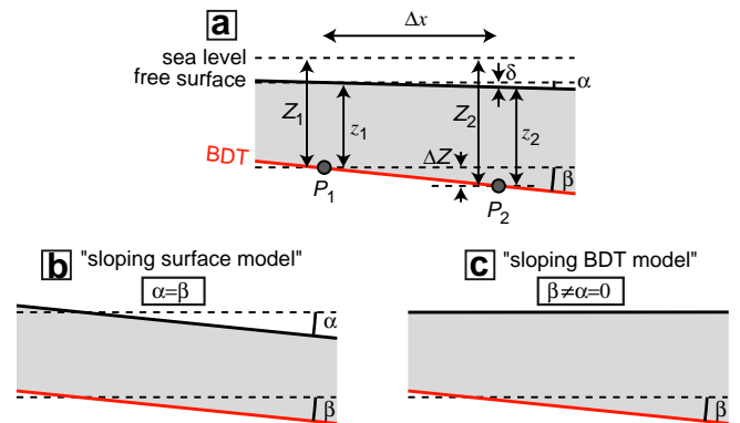
Fig. 5. (a) Geometry of the problem, assuming a migration of magma along the BDT. The free surface and the BDT make an angle \alpha and \beta , respectively, with respect to horizontal. Z is the absolute altitude, i.e. the vertical distance with respect to an arbitrary horizontal level, such as sea level. z is the depth below the free surface, i.e. the height of the overlying column of rock. (b) “Sloping surface model”. (c) “Sloping BDT model”.
