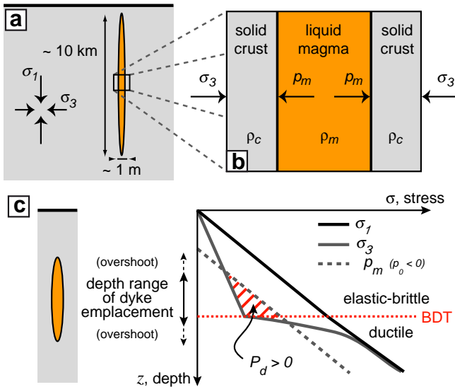
Fig. 3. (a) Cross-section of a dyke intrusion, perpendicular to its along-strike direction. (b) Blow-up of the magma-filled dyke, showing the stress components acting normal on the crack surface. Orange: magma (dyke interior). Grey: host rock (dyke exterior). (c) Stress as a function of depth when differential stress \sigma_d follows the yield envelope ("faulting stress case"). The magnitude of \sigma_d (defined as \sigma_d = \sigma_3 - \sigma_1 < 0 ) is minimum (i.e. relative tension is maximum) at the brittle–ductile transition (BDT). The area hatched in red indicates the region of positive driving pressure P_d , i.e. where magma pressure exceeds the horizontal least compressive principal stress (magma pressure above and below this region is extrapolated). Dyke intrusion preferentially occurs in this depth range, although actual dyke height can be greater due to elastic deformation of host-rock near dyke top and bottom. The cross-sectional shape of the dyke shown here is schematic. Note that the dyke shown here does not reach the surface, which corresponds to a negative magma overpressure p_0 . (For interpretation of the references to colour in this figure legend, the reader is referred to the web version of this article.)
