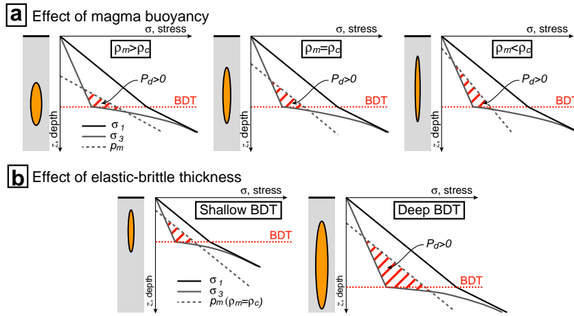
Fig. 4. Effect of (a) magma buoyancy, and (b) depth of the brittle–ductile transition (BDT) on the depth and aspect ratio of dyke intrusions. The cross-sectional shape of the dykes shown here is schematic.
