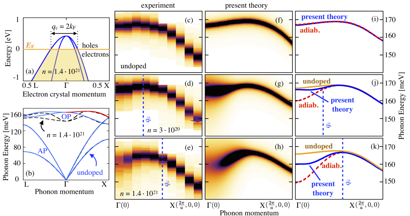
Figure 1. (a) Density-functional theory band structure of diamond for a B concentration of 1.4 \cdot 10^{21} \text{ cm}^{-3} . (b) Adiabatic phonon dispersions of pristine (blue lines) and B-doped diamond (dashed black lines) for momenta along L- \Gamma -X, as obtained from density-functional perturbation theory. (c)-(e) Measured IXS spectra of pristine and B-doped diamond. The critical momentum for the onset of the KA, q_c = 2k_F , is indicated by vertical dashed lines, see also (a). (f)-(h) Non-adiabatic spectral function, obtained from Eqs. (1)-(2), for the LO phonon of (c) pristine and (d)-(e) B-doped diamond along \Gamma -X. The phonon branch considered here is marked by the red line in panel (b). (i)-(k) Phonon energies obtained from Eq. (3) in the adiabatic approximation ( \Pi_{\mathbf{q}\nu}^{\text{NA}} = 0 ), and from the fully non-adiabatic theory (present theory). Non-adiabatic phonon dispersions of undoped diamond are reported for comparison. All doping concentrations are in units of \text{cm}^{-3} .
