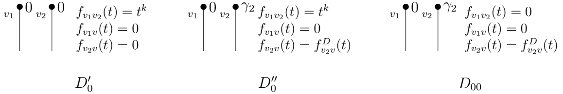
Figure 17: The diagrams D'_0 , D''_0 and D_{00} , with v \neq v_1, v_2 .
