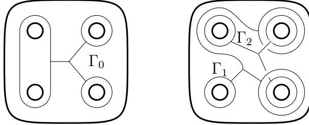
Figure 9: Topological equivalence for leaf cutting
