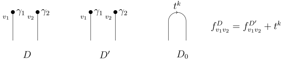
Figure 16: The diagrams D , D' , and D_0 , where \gamma_1, \gamma_2 \in \mathfrak{A} and k \in \mathbb{Z} .
