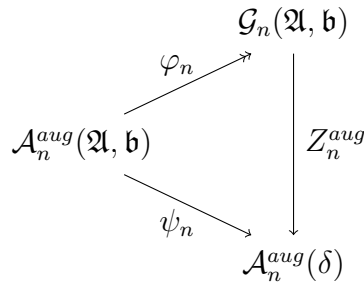
Figure 1: Commutative diagram
