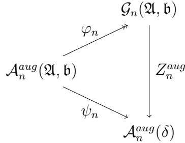
Figure 1: Commutative diagram
