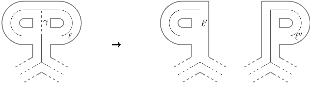
Figure 10: Cutting a leaf
