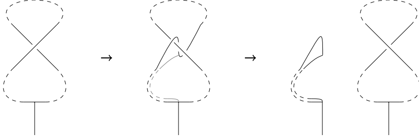
Figure 11: Self-crossing of a leaf
