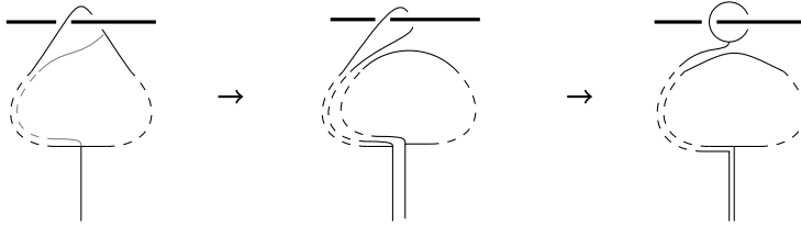
Figure 12: Crossing of an edge or a leaf
