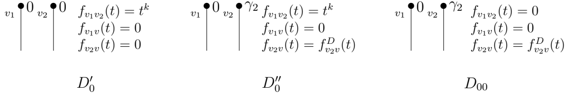
Figure 17: The diagrams D'_0 , D''_0 and D_{00} , with v \neq v_1, v_2 .
