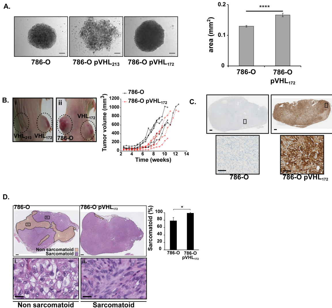
Figure 2: Tumorigenic effect 786-O-pVHL 172 cell-derived tumors compared with 786-O cell-derived tumors. (A) Morphology of 786-O, 786-O-pVHL 213 and 786-O pVHL 172 spheroids (left panels). Spheroid areas from 786-O and 786-O-pVHL 172 cells were measured with the ImageJ software (right histogram, mean±sem, n=58 and n=45 respectively; Mann-Whitney test, ****: p<0.0001). Scale bars: 100 μm. (B) External morphology of tumors obtained by xenografting 786-O-pVHL 172 de mice (i-left flank and ii-right flank), 786-O-pVHL 213 (i-right flank) or 786-O cells (ii-left flank) in nude mice. Growth kinetics of 786-O and 786-O-pVHL 172 derived tumors determined by measuring the tumor volumes using a caliper (n=5 tumors per cell type). (C) pVHL 172 expression was controlled by immunohistochemical staining with an anti-HA antibody in 786-O-pVHL 172 and 786-O cell-derived tumors (upper panels; scale bar: 500μm). A 20X magnification is shown in the lower panels (scale bar: 100μm). (D) Sarcomatoid and non-sarcomatoid areas were delimited following HE staining of 786-O and 786-O-pVHL 172 cell-derived tumor sections (upper panels, scale bar: 500μm). Inserts in a representative 786-O tumor section show the gradual progression of the tumor phenotype from (i) non-sarcomatoid morphology to (ii) a tissue with sarcomatoid component (scale bar: 20μm). The histogram shows the percentage of sarcomatoid areas relative to the whole tumor section (mean ± s.d., n=5 tumors/cell type; Mann-Whitney test: p<0.05).
