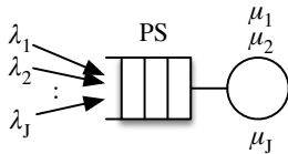
Fig. 1: PS queue model
