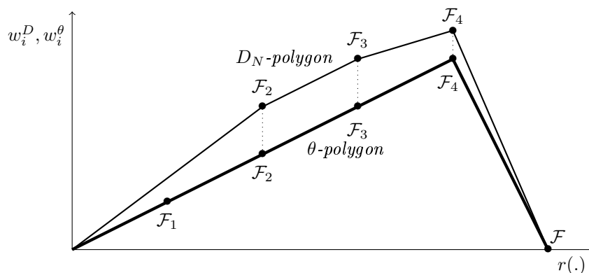
FIGURE 4. \theta -polygon and D_N -polygons of Example 4.4
