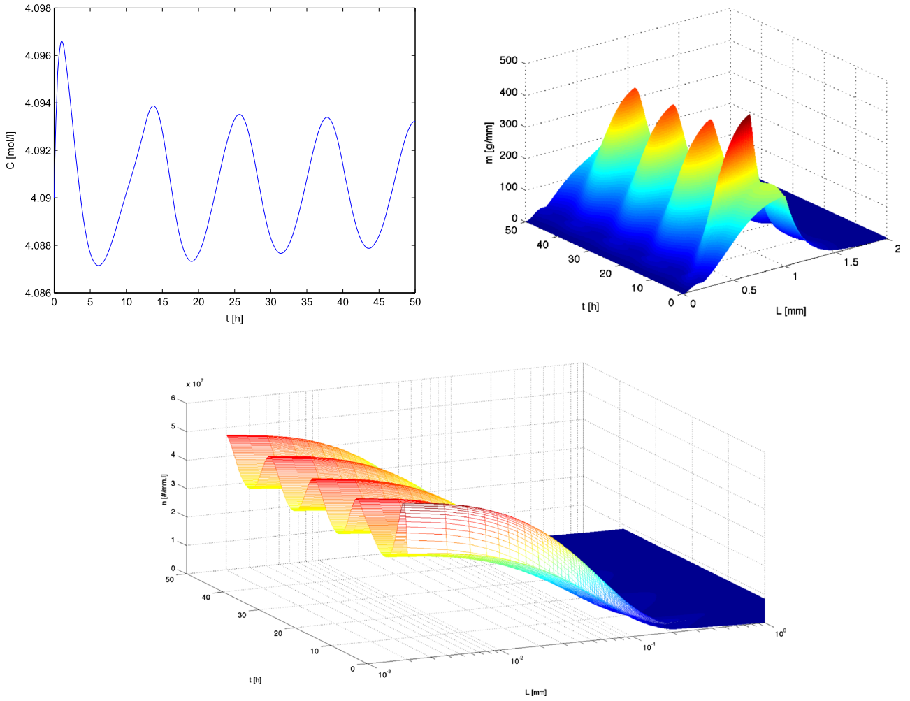
Figure 2. Simulation of continuous crystallizer with fines dissolution, product removal, and negligible attrition at steady state. Solute concentration (left), mass density m(L, t) = \rho k_v n(L, t) L^3 (right), and number density function n(L, t) (at the bottom) show sustained oscillations and even instability, which may degrade product quality.
