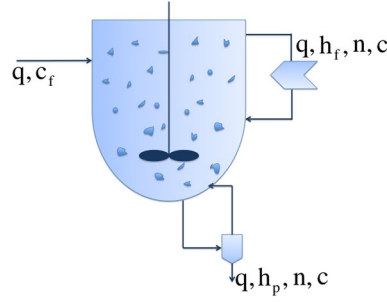
Figure 1. Continuous KCl crystallizer [23] filled with liquid (solute and solvent) and solids (crystals). Internal processes are nucleation, growth, attrition and breakage, and possibly agglomeration. External phenomena include solute feed c_f at rate q (upper-left), recycling of fines h_f (upper-right), product removal h_p (lower-right), stirring, and possibly heating or cooling to act on the saturation concentration c_s .
