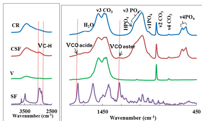
Fig. 2. FTIR spectra of sodium fusidate (SF), vaterite (V), reference cement (CR), and SF-loaded cement (CSF).
