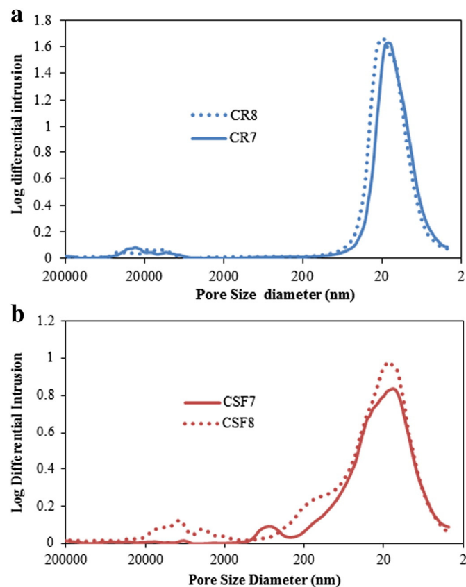
Fig. 4. Pore-size distribution of the reference (a) and the SF-loaded (b) cements, both prepared with L/P ratios of 0.7 and 0.8.
