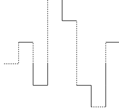
Figure 1: Microscopic disorder \omega in the copolymer. Dashed bonds represent monomers of type A (hydrophobic), drawn bonds represent monomers of type B (hydrophilic).
