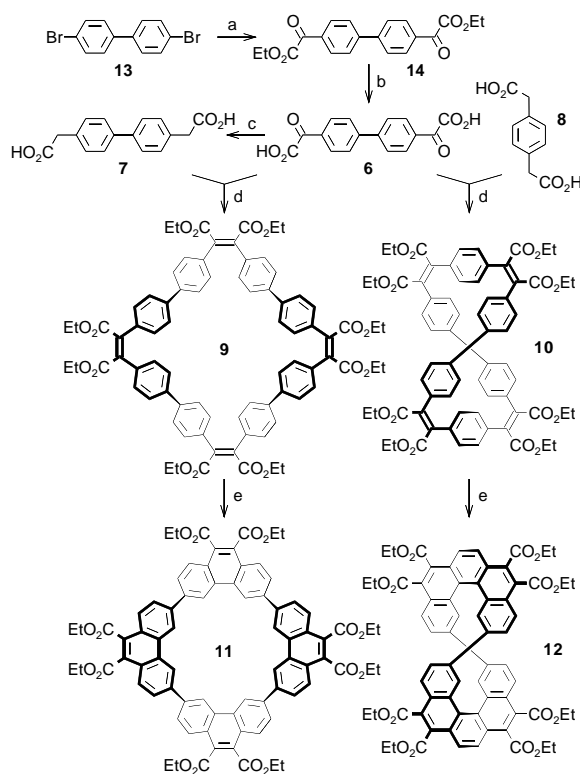
Scheme 3. Synthesis of saddle-shaped tetra-3,6-phenanthrylene-octaester 11 and propellcene-octacarboxylate 12 . (a) 1. THF, n -BuLi, 2. \text{EtO}_2\text{CCO}_2\text{Et} , 62%; (b) \text{NaHCO}_3 , EtOH- \text{H}_2\text{O} , 100%; (c) NaI, \text{H}_3\text{PO}_2 , \text{H}_2\text{O} , AcOH, 94%; (d) 1. \text{NEt}_3 , \text{Ac}_2\text{O} , THF (high dilution), 2. EtOH, EtBr, DBU, 52% ( 9 ) / 21% ( 10 ); (e) h\nu , \text{I}_2 , \text{O}_2 , EtOAc-dioxane or PhMe, 47% ( 11 ) / 54% ( 12 ).
