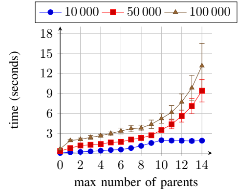
Fig. 8. Learning time according to the maximum number of parents per variable. Dataset is randomly generated (15 variables, \delta = 0.95 ) with varied number of comparisons (one per graphic line).
