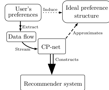
Fig. 1. Global scheme of a learning procedure for CP-nets.
