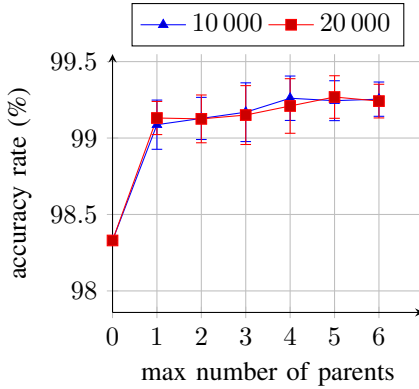
Fig. 9. Learning accuracy according to the maximum number of parent per variable from real datasets. For each dataset, we select two different number of pairwise comparisons.
