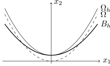
Figure 1: Graph of \Omega , \Omega_h , and B_h for \varphi(x_1) = \|x_1\|^2 and h = 0.5
