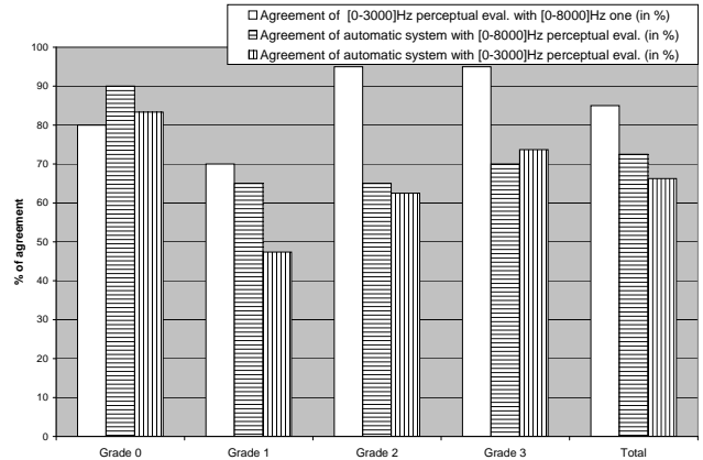
Figure 3: Agreement rate (in %) between both [0-3000]Hz and [0-8000]Hz perceptual evaluation and between automatic grade classification and perceptual evaluations.
