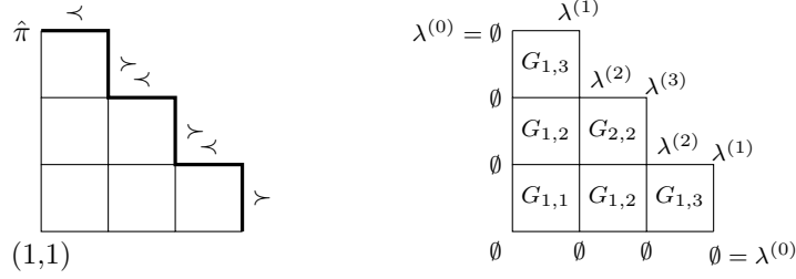
Figure 7: Left: the encoded shape sh(w^{\text{sym}}) = (3, 2, 1) for w = (\prec, \succ, \prec) together with the down-right path \hat{\pi} in bold; right: the partitions \lambda^{(0)}, \dots, \lambda^{(3)}, \dots, \lambda^{(0)} associated to the points of \hat{\pi} are constructed recursively using the empty partitions on the boundary, the G_{r,t} and \mathcal{T}_{\text{loc}} .
