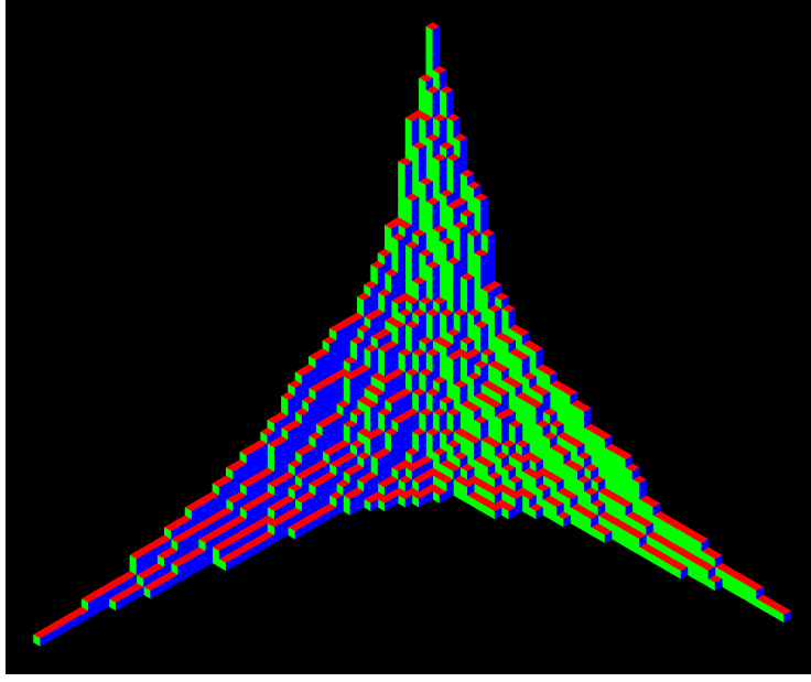
Figure 17: A large random plane overpartition shown as a strict plane partition.
