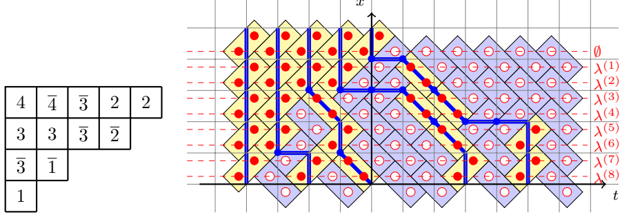
Figure 5: A plane overpartition (left) and its associated point configuration (right).
