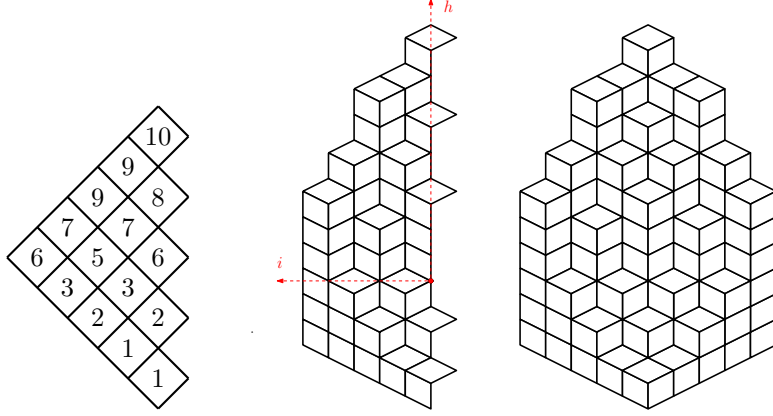
Figure 9: Left: a free boundary plane partition \pi of length 5, with \pi_{1,1} = 10, \pi_{4,2} = 5, \dots , corresponding to interlacing partitions \emptyset \prec (6) \prec (7, 3) \prec (9, 5, 2) \prec (9, 7, 3, 1) \prec (10, 8, 6, 2, 1) ; middle: a stack of cubes depicting \pi via the heights of the horizontal lozenges; right: the corresponding symmetric plane partition with base contained in a 5 \times 5 square.
