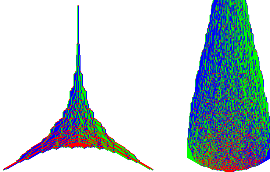
Figure 4: Large unbounded (left) and bounded (right) random symmetric q^{\text{Volume}} -weighted plane partitions.
