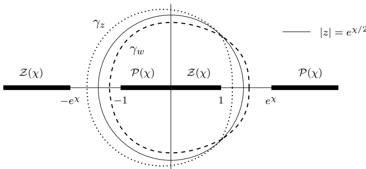
Figure 16: Deformed contours in z and w .
