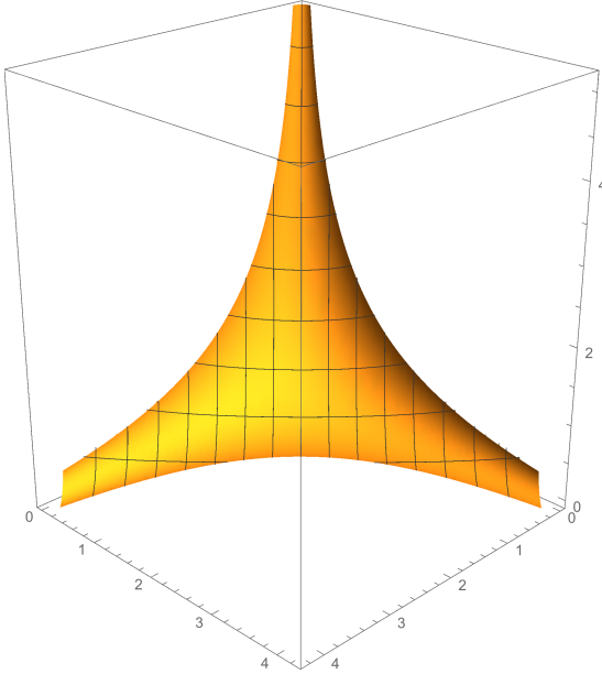
Figure 13: The limit surface for both symmetric and non-symmetric random plane partitions.
