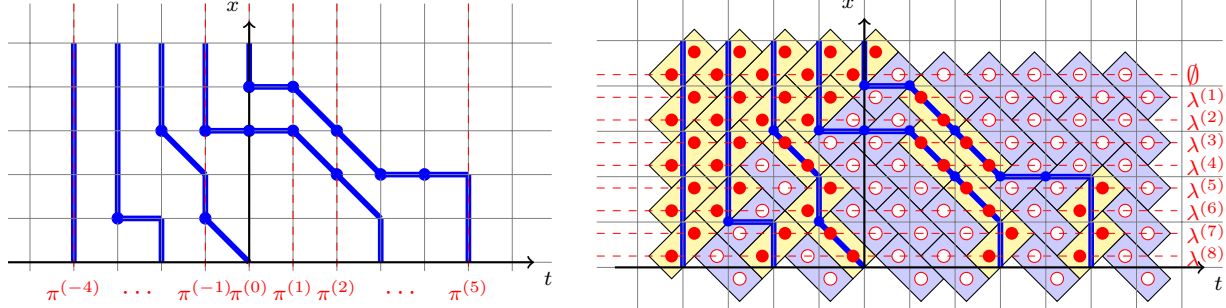
Figure 15: Strict plane partition point configuration (left) and plane overpartition point configuration (right).
