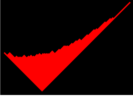
Figure 2: A random partition \lambda , in Russian notation, whose weight is proportional to s_\lambda(q, \dots, q) (100 q 's) for q = 1/3 . The right arm (its first part) is, via the RSK correspondence, the last passage percolation time in a 100 \times 100 symmetric matrix filled with otherwise independent geometric random numbers of parameter q^2 (off diagonal) and q (on the diagonal).
