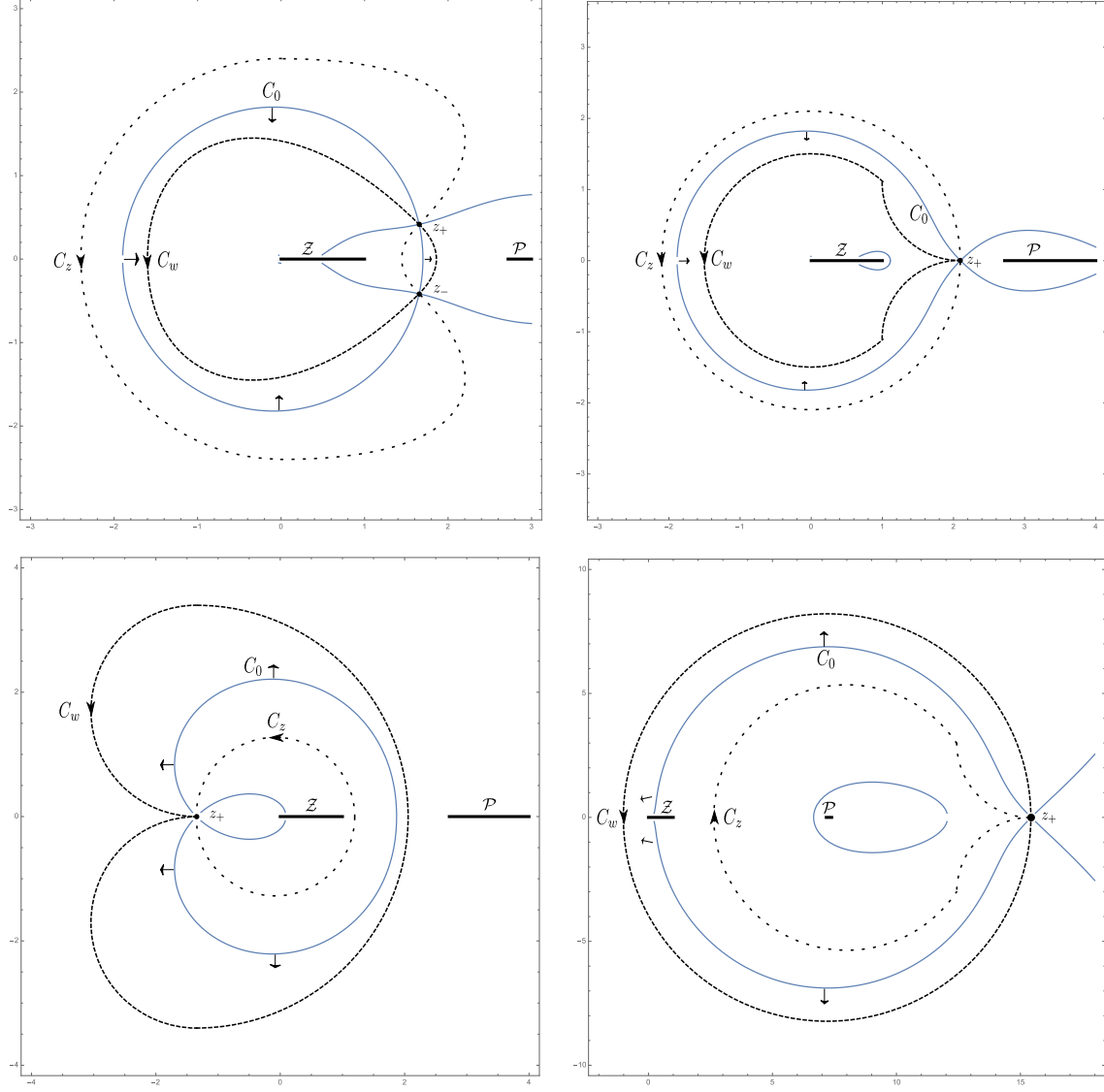
Figure 12: The curves (solid) \Re(S(z) - S(z_+)) = 0 with arrows in the direction of ascent and the final z and w contours from the proof of Theorem 5.6. Top left: z_+ is one of the two complex conjugate critical points of S corresponding to the liquid region; top right: z_+ is real corresponding to the region above the arctic curve; bottom left: z_+ is real and corresponds to the region below the arctic curve and \chi < \chi_T ; bottom right: like bottom left but with \chi > \chi_T .
