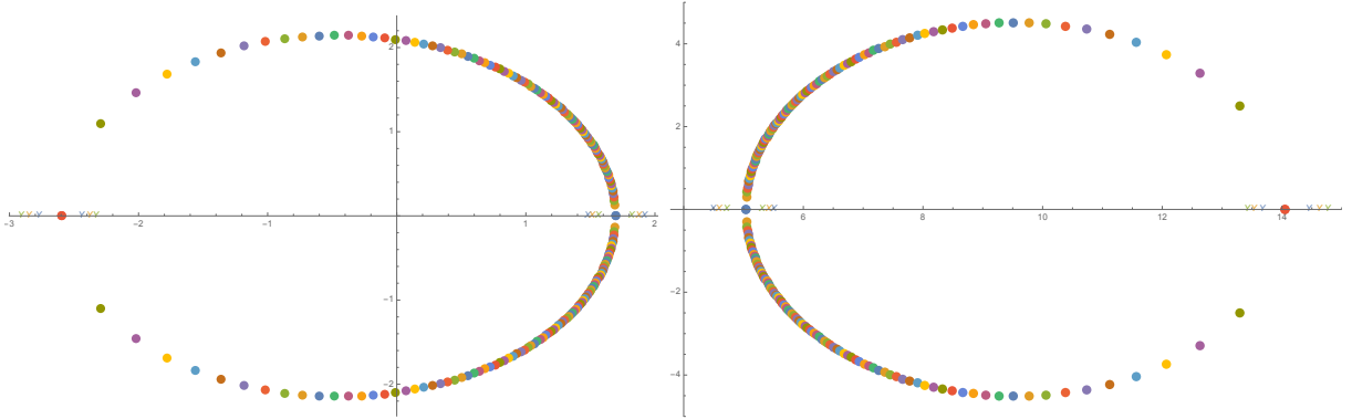
Figure 11: The critical points of S , for a = 2 and for \chi = 1 < \chi_T (left), \chi = 1.97 > \chi_T (right) fixed, as y varies from just above y_+ to just below y_- ; they are distinct real for y > y_+ (denoted by an X) approaching the double critical point at y = y_+ ; they are complex conjugate for y_+ > y > y_- approaching the double critical point at y = y_- and they become distinct real again (denoted by Y) diverging from said double critical point as y decreases below y_- .
