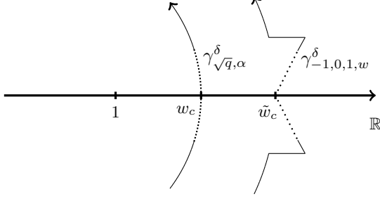
Figure 8: Parts of the contours \gamma_{\sqrt{q},\alpha} and \gamma_{-1,0,1,w} from (4.38) and (4.42) close to where they cross the positive real axis in w_c = 1 + N^{-1/3}(2|v|c_q + 1/2) , \tilde{w}_c = w_c + N^{-1/3}/2 . The curve segments \gamma_{\sqrt{q},\alpha}^\delta, \gamma_{-1,0,1,w}^\delta are shown in dotted lines.
