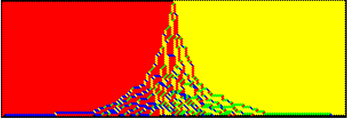
Figure 6: A large random plane overpartition shown as a domino tiling.
