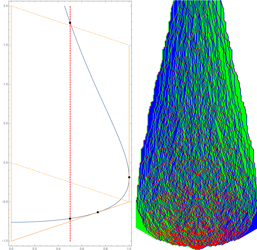
Figure 10: Left: a portion of the arctic curve for a = 1 in the lozenge (\chi, \hat{h}) = (\chi, y - \chi/2) coordinates; the vertical dashed line is of abscissa \chi = 1/2 and intersects the arctic curve in the two points \hat{h}_{\pm} = y_{\pm} - \chi/2 ; the points of tangency of the arctic curve to the boundary of the domain on the bottom and right are also pictured. Right: a simulation (after symmetrization) of a boxed plane partition with base of size 100 \times 100 and q \approx 0.98 using the algorithm from [BBB + 15].
