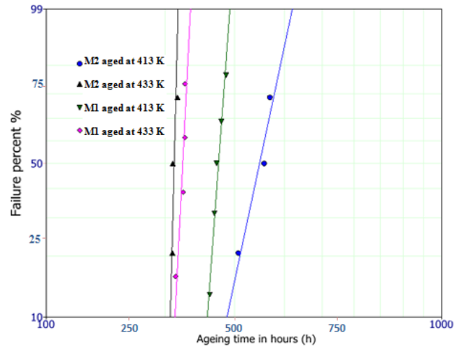
Fig. 14. Weibull probability plots vs aging time.
