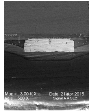
Fig. 17. View of the contact between Antenna/RFIC without failures.
