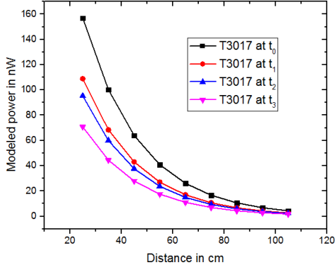
Fig. 9. Modeled reflected power of T3017 aged at 413 K vs distance.
