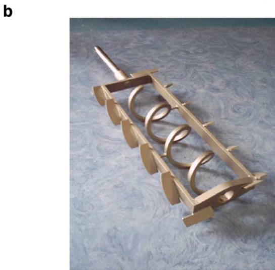
Fig. 1. (a) - GCM500 mixing system including loss-in-weight feeders, inlet chute, mixer body ; (b) - Stirrer type used in the present study showing the frame supporting the blades and the internal transport screw.
