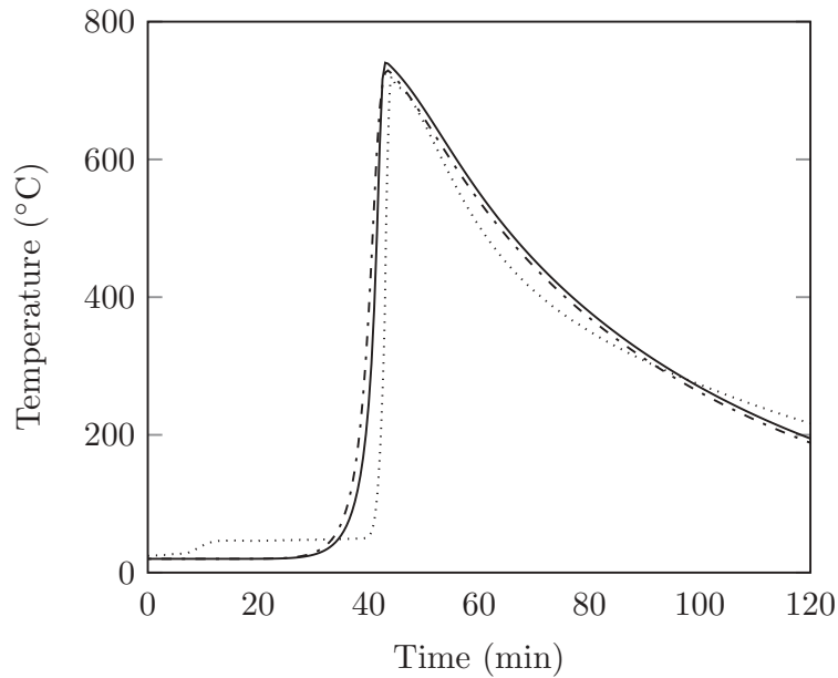
Figure 7. Temperature history on the revolution axis at 19 cm from the inlet. Continuous line: model solid temperature; dashed line: model gas temperature, model; dotted line: experimental observations. C = 2.3\% , Pe = 1.6 .
