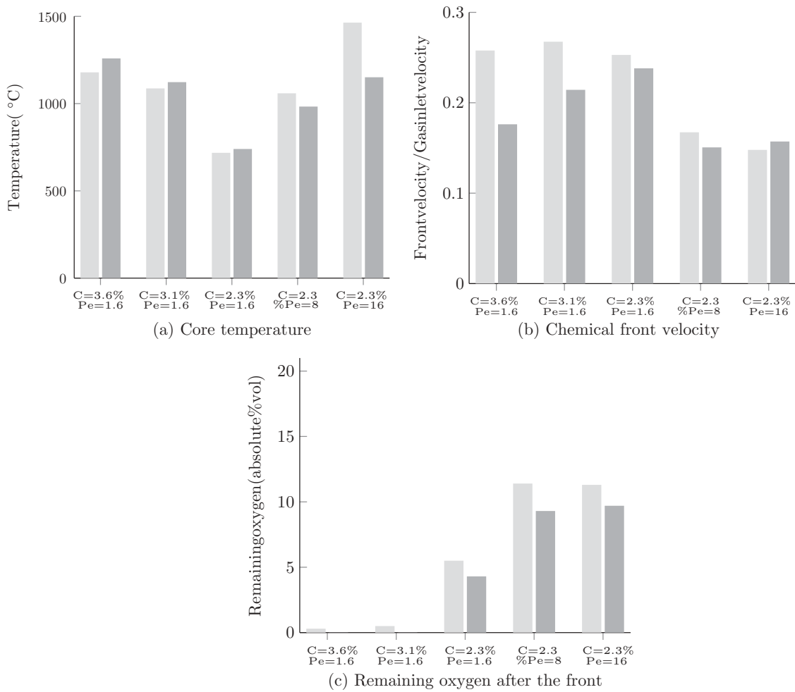
Figure 4. Experimental observation and numerical predictions. Light gray: experimental observations; dark gray: numerical predictions.
