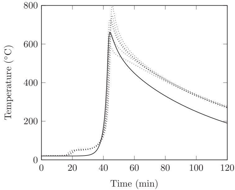
Figure 8. Solid temperature history 1 cm away from the wall at 19 cm from the inlet. Continuous line: model; dotted line: experimental observations. C = 2.3\% , Pe = 1.6 .
