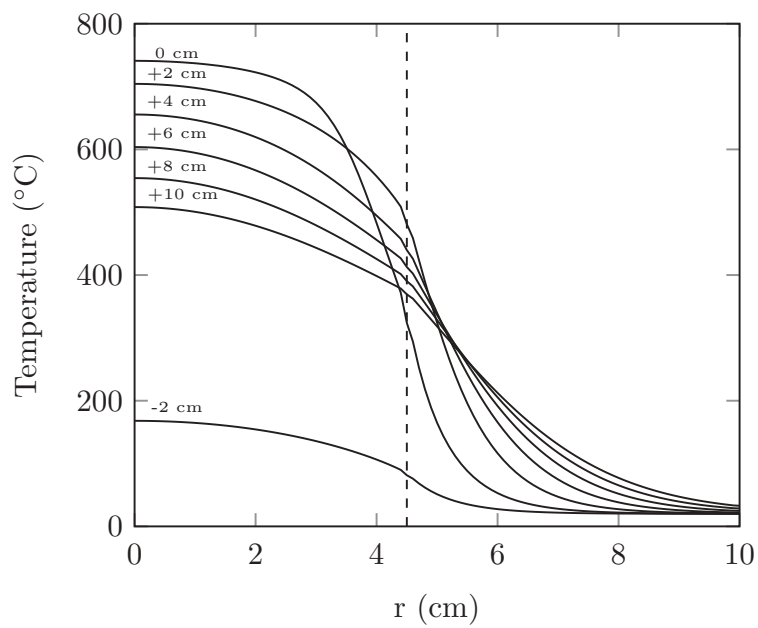
Figure 6. Solid temperature profiles after 1 h at various locations relative to the front (Figure 5). Front position: 29 cm. C = 2.3\% , Pe = 1.6 .
