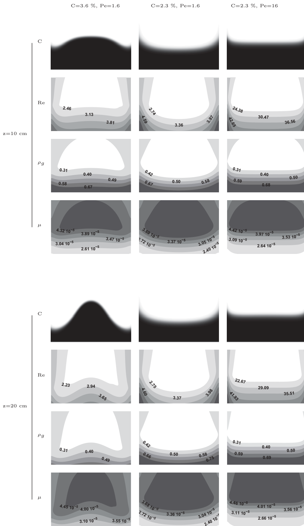
Figure 11. Different fronts shapes, viscosity, density, and Reynolds number maps observed in the reference case (center), with high carbon content (left) and with high gas velocity (right). Color legend: the darker, the higher.
