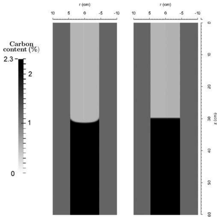
Figure 10. Carbon field inside of the combustion cell when half of the medium has been consumed. On the left: with heat loss. On the right: without the heat loss. Color legend: the darker, the higher.
