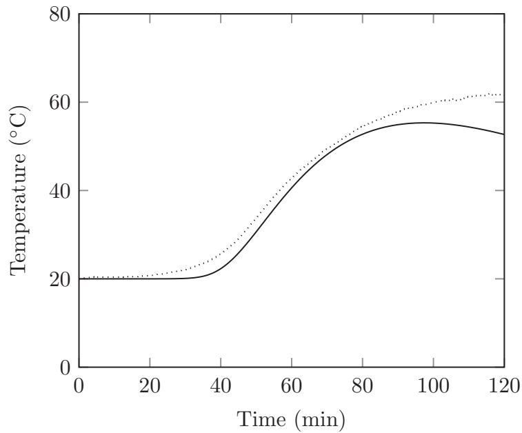
Figure 9. Superimposition of the solid temperature histories on outer surface of the cell at 19 cm from the inlet. Continuous line: model; dotted line: experimental observations.
