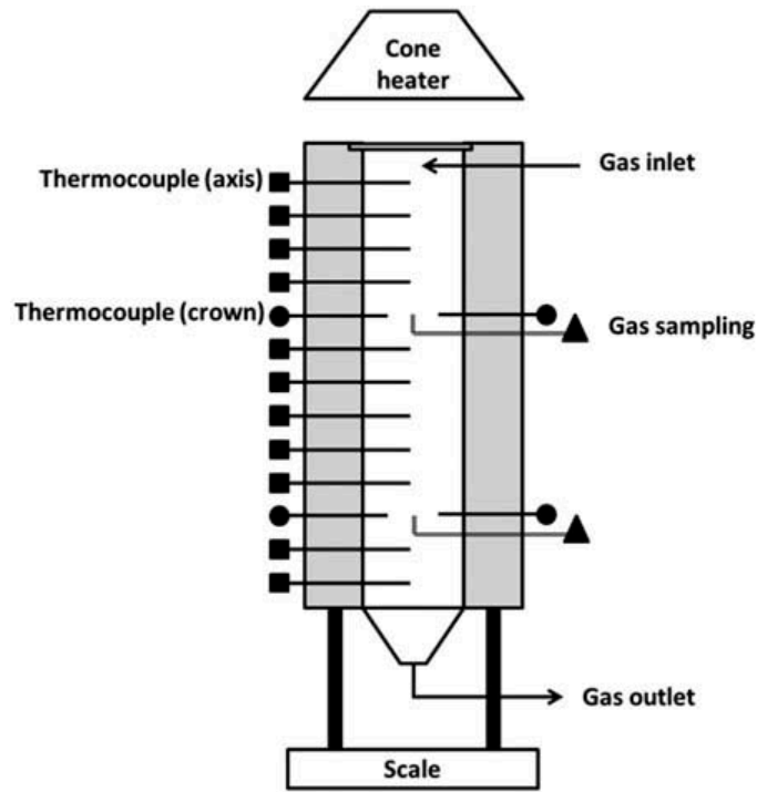
Figure 1. Schematic of the experimental apparatus. [Reprinted with permission from G. Baud, S. Salvador, G. Debenest, and J.-F. Thovert. 2015. New granular model medium to investigate smoldering fronts propagation—Experiments. Energy & Fuels , 29(10), 6780–6792. Copyright 2015 American Chemical Society.]
