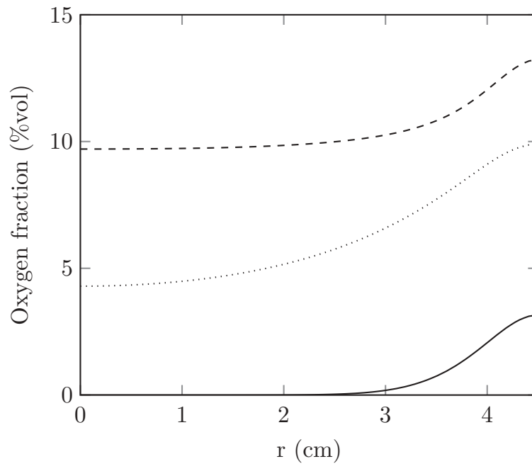
Figure 12. Remaining oxygen downstream of the front. Continuous line: C = 3.6\% , Pe = 1.6 ; dotted line (reference case): C = 2.3\% , Pe = 1.6 ; dashed line: C = 2.3\% , Pe = 16 .
