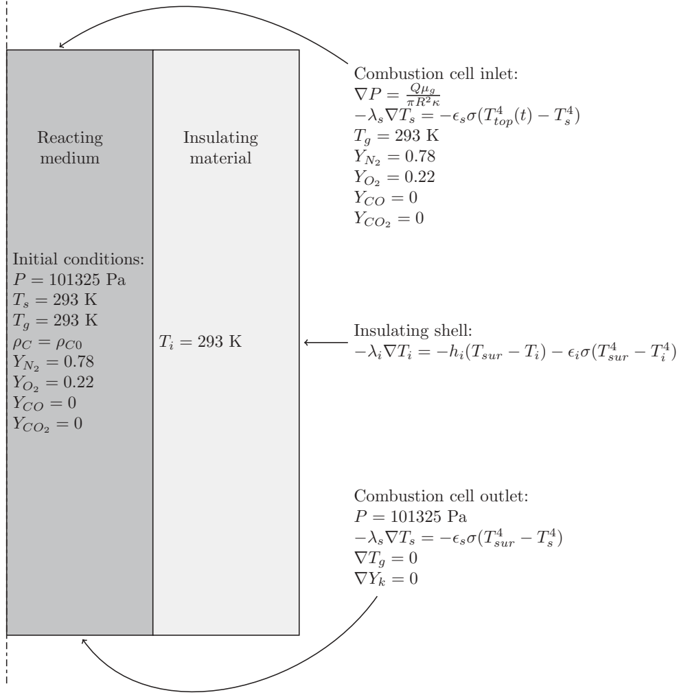
Figure 2. Numerical domain schematic with boundary conditions.
