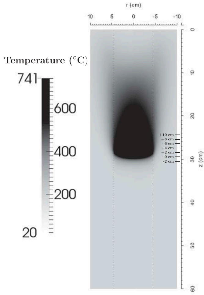
Figure 5. Solid temperature field inside of the combustion cell after 1 h. C = 2.3\% , Pe = 1.6 . Locations marked: position relative to the chemical front (as used in Figure 6).
