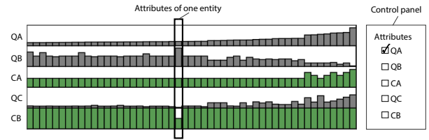
Fig. 1. A HEDA with 5 attributes ( \{QA, QB, CA, QC, CB\} ) using size to encode their values: green for categorical; gray for quantitative attributes.
