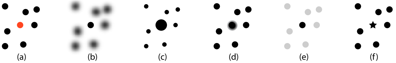
Figure 8: An emphasis effect created in a scatterplot by using (a) highlighting in red, (b) blurring, (c) size/area, (d) depth, (e) transparency / value, and (f) shape. In all cases, only one data point is emphasized, e.g., in (a) F is the only data point coloured red, B is the set of black data points, and M = \emptyset .
