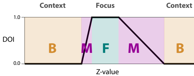
Figure 6: This image is a facsimile that we have created to emulate the one-dimensional trapezoidal DOI function of Doleisch et al. [DHGK06]. The z values represent some attribute of the data points. Assuming that the visualization shows all of the data points, the z value of a data point determines whether it is part of the focus ( DOI = 1 ) and therefore in F ; part of the context ( DOI = 0 ) and in B ; or somewhere in between ( 0 < DOI < 1 ) and therefore in M .
