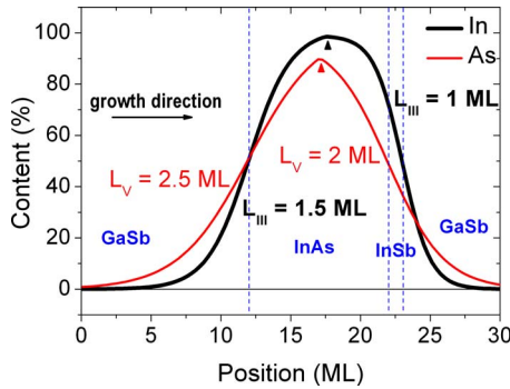
FIG. 3. (Color online) Composition profiles across a (10 ML GaSb/10 ML InAs/1 ML InSb) SPSL showing (i) chemically broad interfaces and (ii) a different intermixing at the III- and V-element sublattice. The small shift in the distribution profiles for In and As is considered as an indirect evidence of the presence of the 1 ML InSb layer (arrows: indicate points at which the interface profiles are joined).
