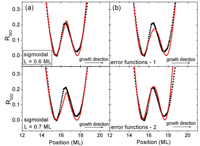
FIG. 2. (Color online) Magnification of the interface-related features in the intensity profile displaying (a) the sensitivity of the method to variations in the interface width as small as 0.1 ML, and (b) the results assuming element profiles based on error functions.
