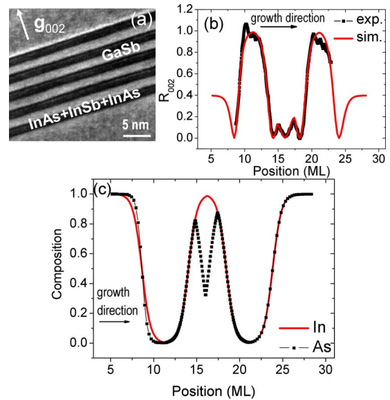
FIG. 4. (Color online) (a) g_{002} DF TEM image of the few ML thick (6 ML GaSb/2 ML InAs/1.5 ML InSb/2 ML InAs) SPSL, (b) simulated intensity profile that agrees best with the experimental results obtained after the composition profiles shown in (c).
