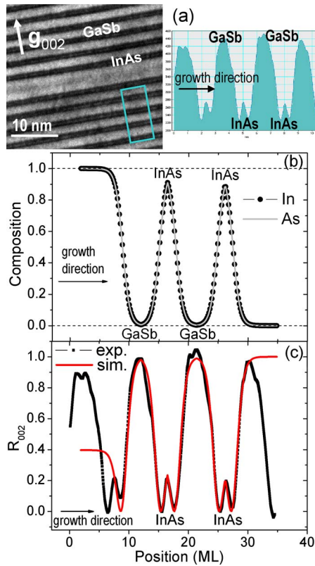
FIG. 1. (Color online) (a) g_{002} DF TEM micrograph of a (3 ML InAs/6 ML GaSb) SPSL, together with an intensity linescan. (b) Proposed element distribution profiles yielding to the simulated R_{002} best reproducing the experimental intensity ratio (c).
